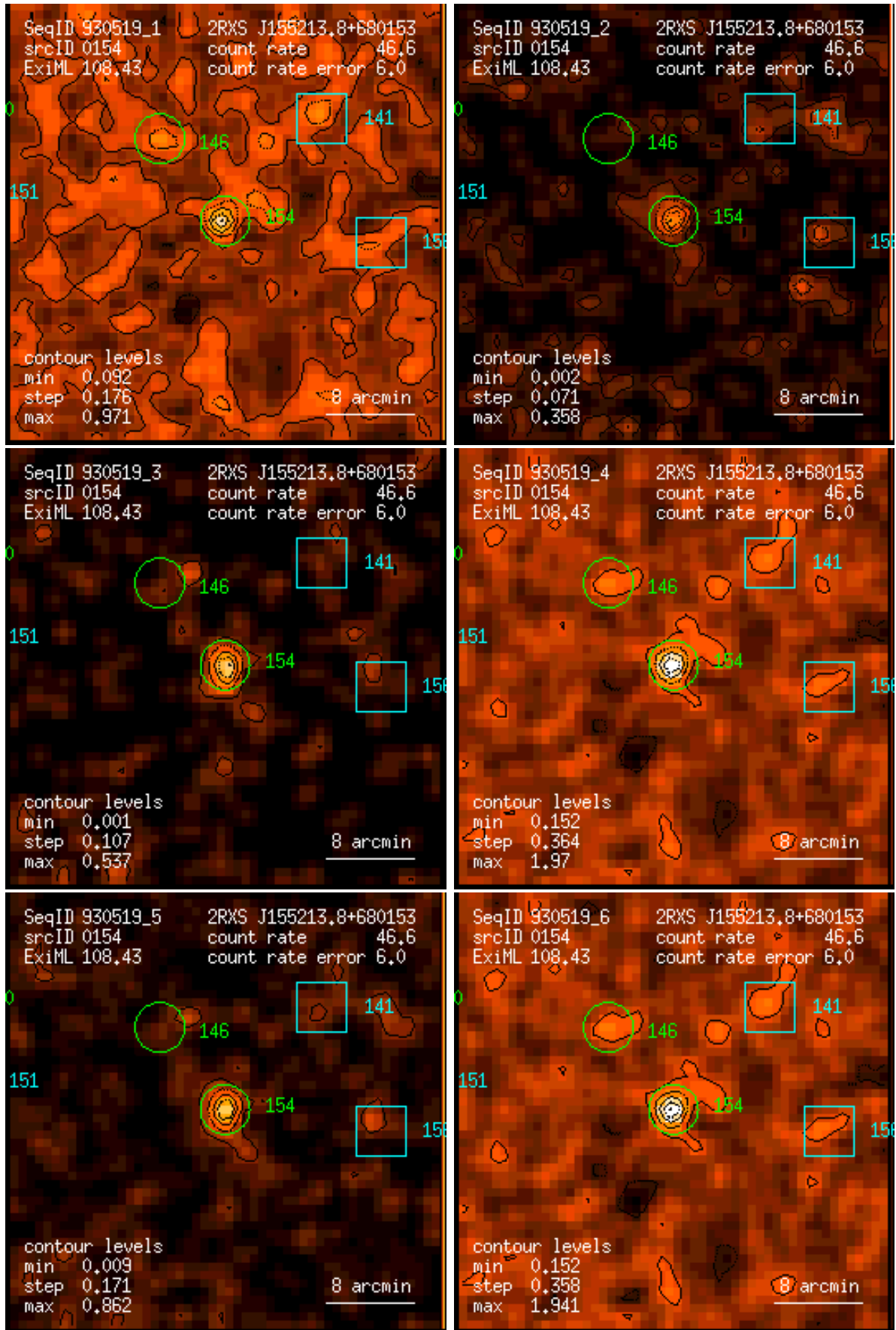
Figure 154: RASS 930519: detection 0154: band rate images, Gaussian filter: (1) PSPC channels 11 – 41, (2) 52 – 90, (3) 91 – 201, (4) 11 – 235, (5) 52 – 201, (6) 11 – 201. Broad band rates in counts/ks. Band rate contour levels in counts/ks/arcmin 2 .
