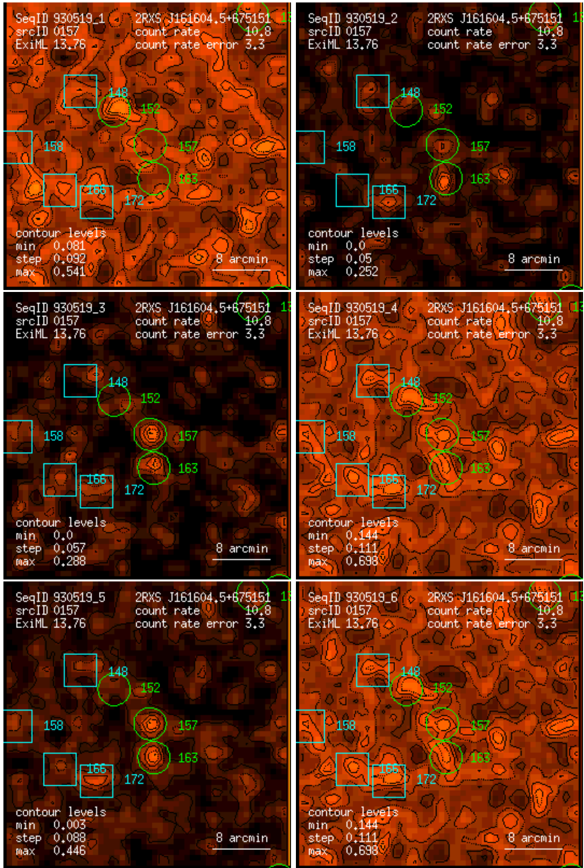
Figure 157: RASS 930519: detection 0157: band rate images, Gaussian filter: (1) PSPC channels 11 – 41, (2) 52 – 90, (3) 91 – 201, (4) 11 – 235, (5) 52 – 201, (6) 11 – 201. Broad band rates in counts/ks. Band rate contour levels in counts/ks/arcmin 2 .
