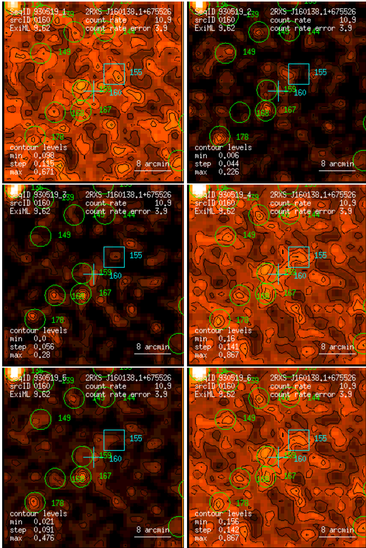
Figure 160: RASS 930519: detection 0160: band rate images, Gaussian filter: (1) PSPC channels 11 – 41, (2) 52 – 90, (3) 91 – 201, (4) 11 – 235, (5) 52 – 201, (6) 11 – 201. Broad band rates in counts/ks. Band rate contour levels in counts/ks/arcmin 2 .
