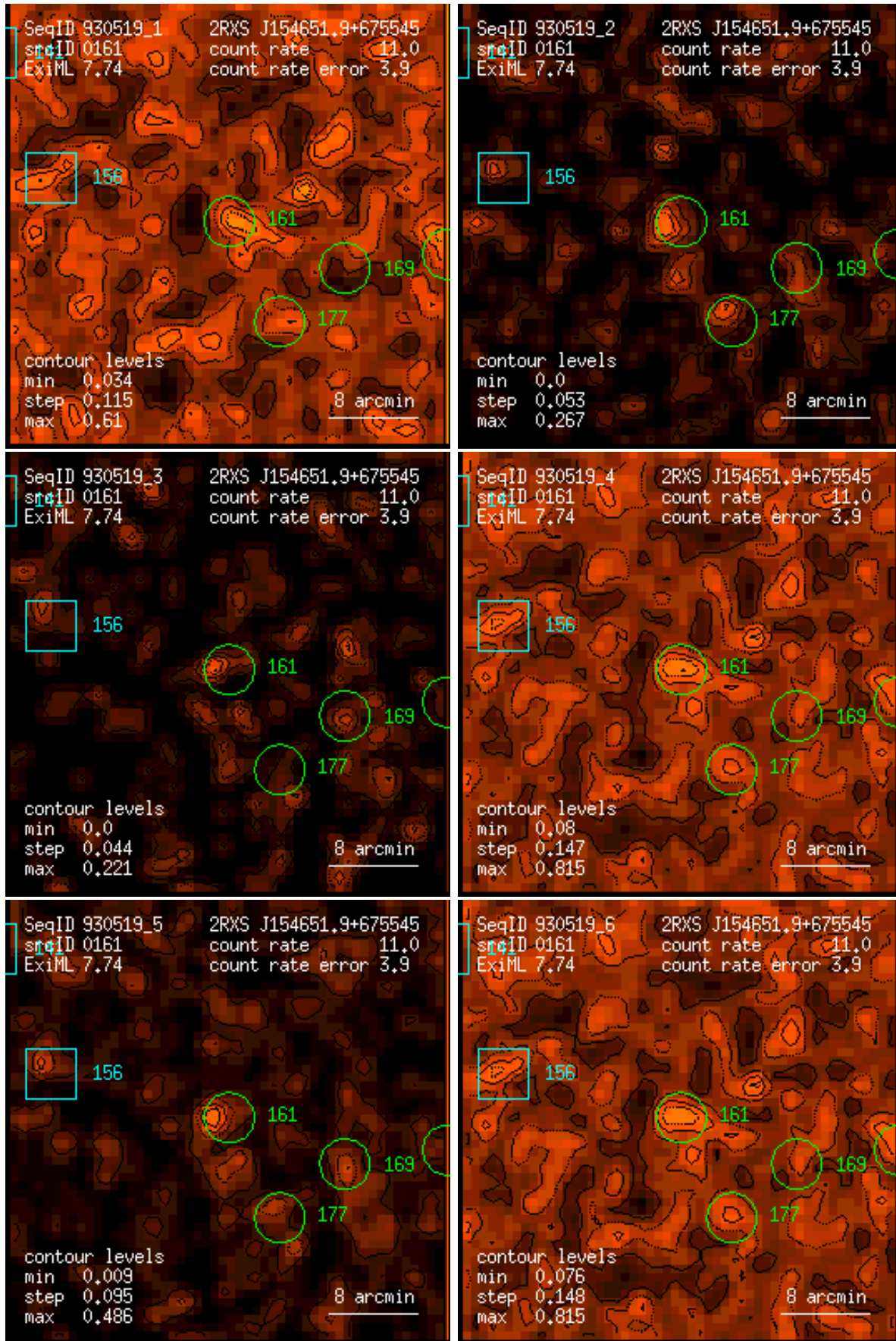
Figure 161: RASS 930519: detection 0161: band rate images, Gaussian filter: (1) PSPC channels 11 – 41, (2) 52 – 90, (3) 91 – 201, (4) 11 – 235, (5) 52 – 201, (6) 11 – 201. Broad band rates in counts/ks. Band rate contour levels in counts/ks/arcmin 2 .
