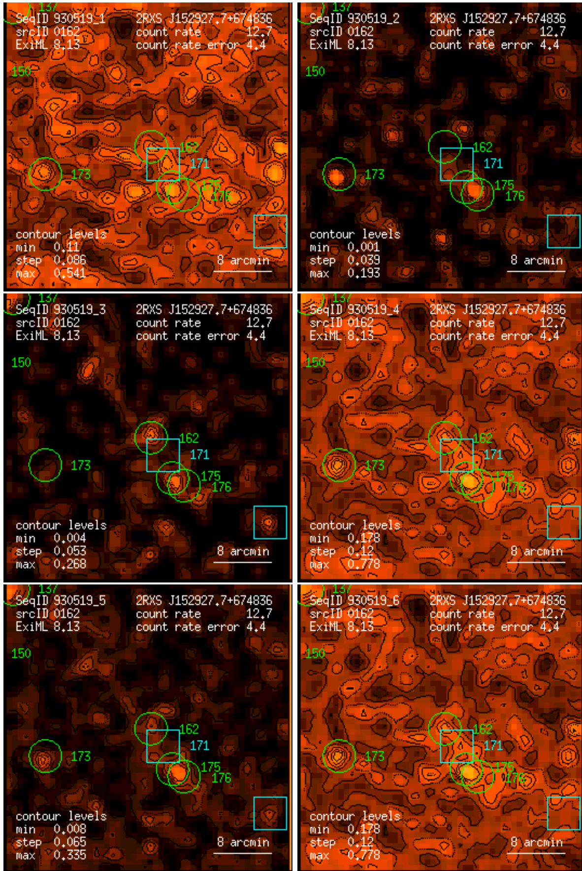
Figure 162: RASS 930519: detection 0162: band rate images, Gaussian filter: (1) PSPC channels 11 – 41, (2) 52 – 90, (3) 91 – 201, (4) 11 – 235, (5) 52 – 201, (6) 11 – 201. Broad band rates in counts/ks. Band rate contour levels in counts/ks/arcmin 2 .
