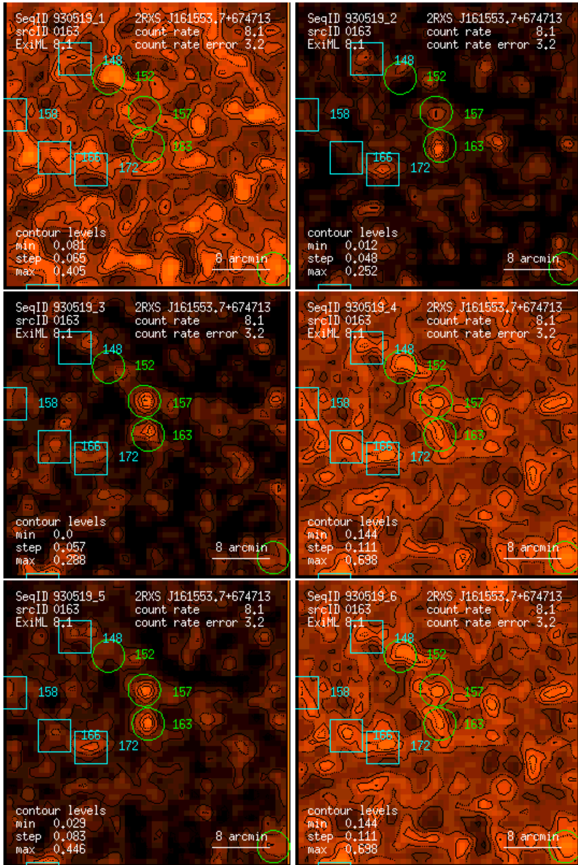
Figure 163: RASS 930519: detection 0163: band rate images, Gaussian filter: (1) PSPC channels 11 – 41, (2) 52 – 90, (3) 91 – 201, (4) 11 – 235, (5) 52 – 201, (6) 11 – 201. Broad band rates in counts/ks. Band rate contour levels in counts/ks/arcmin 2 .
