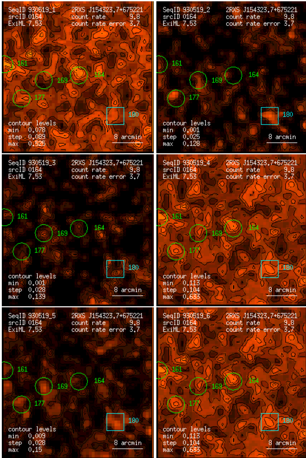
Figure 164: RASS 930519: detection 0164: band rate images, Gaussian filter: (1) PSPC channels 11 – 41, (2) 52 – 90, (3) 91 – 201, (4) 11 – 235, (5) 52 – 201, (6) 11 – 201. Broad band rates in counts/ks. Band rate contour levels in counts/ks/arcmin 2 .
