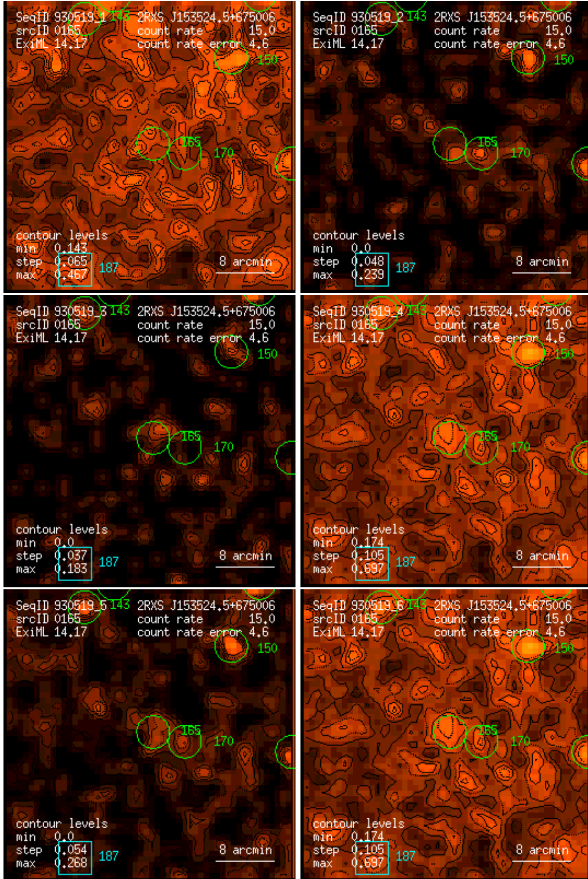
Figure 165: RASS 930519: detection 0165: band rate images, Gaussian filter: (1) PSPC channels 11 – 41, (2) 52 – 90, (3) 91 – 201, (4) 11 – 235, (5) 52 – 201, (6) 11 – 201. Broad band rates in counts/ks. Band rate contour levels in counts/ks/arcmin 2 .
