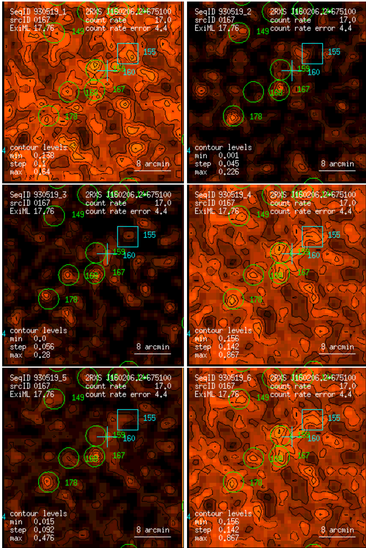
Figure 167: RASS 930519: detection 0167: band rate images, Gaussian filter: (1) PSPC channels 11 – 41, (2) 52 – 90, (3) 91 – 201, (4) 11 – 235, (5) 52 – 201, (6) 11 – 201. Broad band rates in counts/ks. Band rate contour levels in counts/ks/arcmin 2 .
