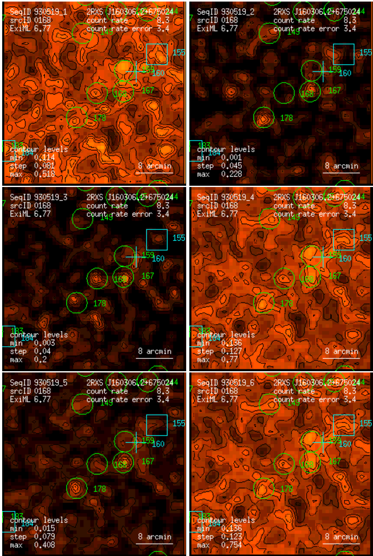
Figure 168: RASS 930519: detection 0168: band rate images, Gaussian filter: (1) PSPC channels 11 – 41, (2) 52 – 90, (3) 91 – 201, (4) 11 – 235, (5) 52 – 201, (6) 11 – 201. Broad band rates in counts/ks. Band rate contour levels in counts/ks/arcmin 2 .
