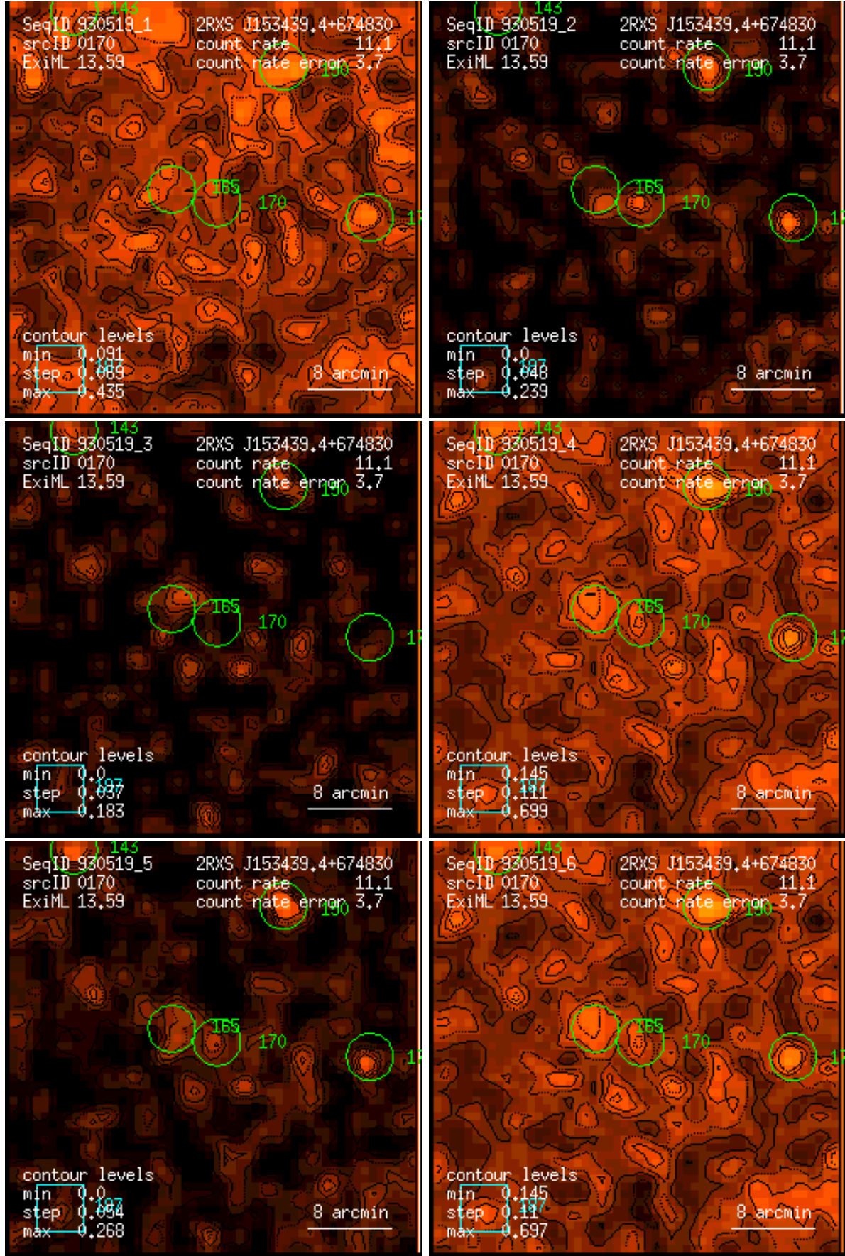
Figure 170: RASS 930519: detection 0170: band rate images, Gaussian filter: (1) PSPC channels 11 – 41, (2) 52 – 90, (3) 91 – 201, (4) 11 – 235, (5) 52 – 201, (6) 11 – 201. Broad band rates in counts/ks. Band rate contour levels in counts/ks/arcmin 2 .
