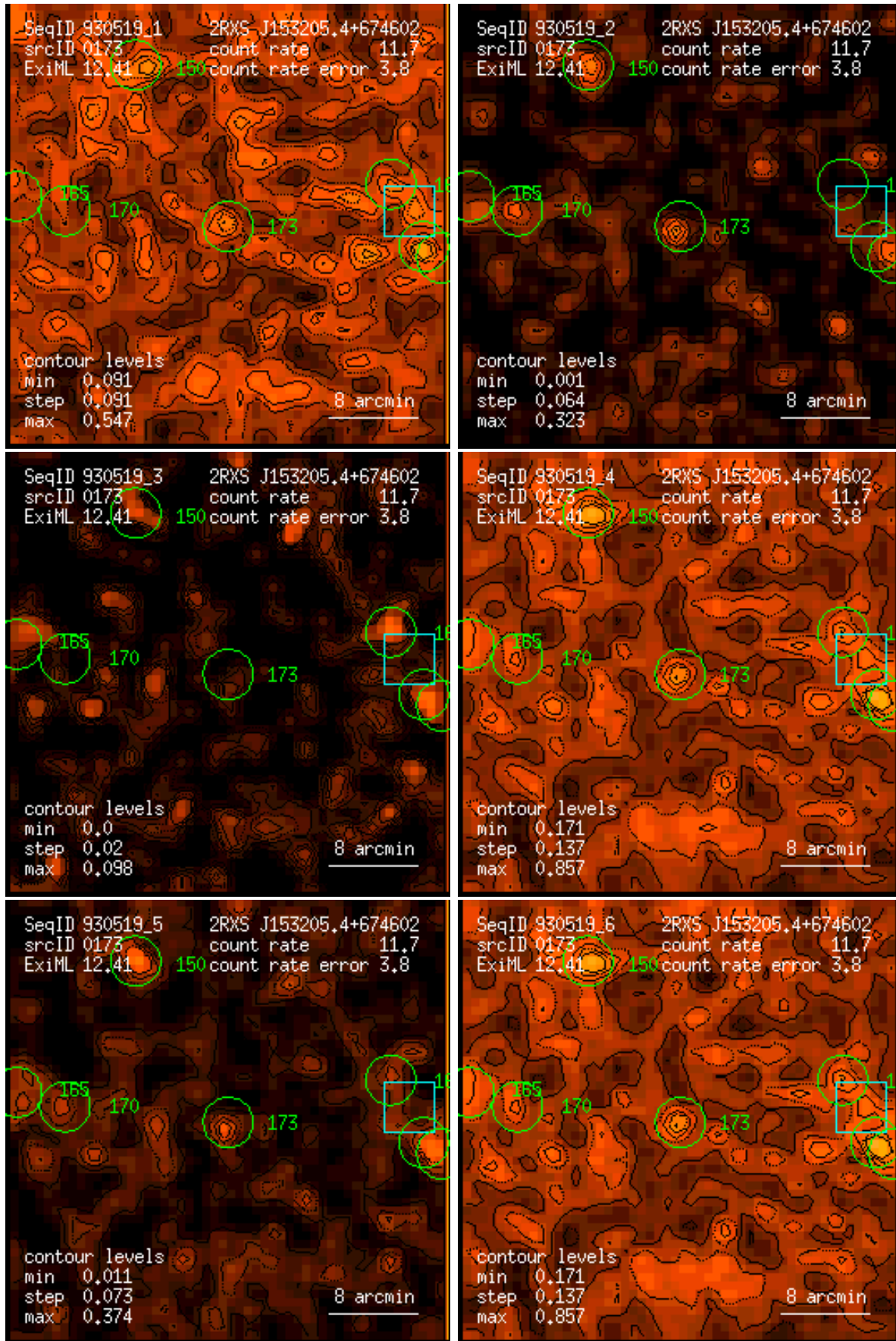
Figure 173: RASS 930519: detection 0173: band rate images, Gaussian filter: (1) PSPC channels 11 – 41, (2) 52 – 90, (3) 91 – 201, (4) 11 – 235, (5) 52 – 201, (6) 11 – 201. Broad band rates in counts/ks. Band rate contour levels in counts/ks/arcmin 2 .
