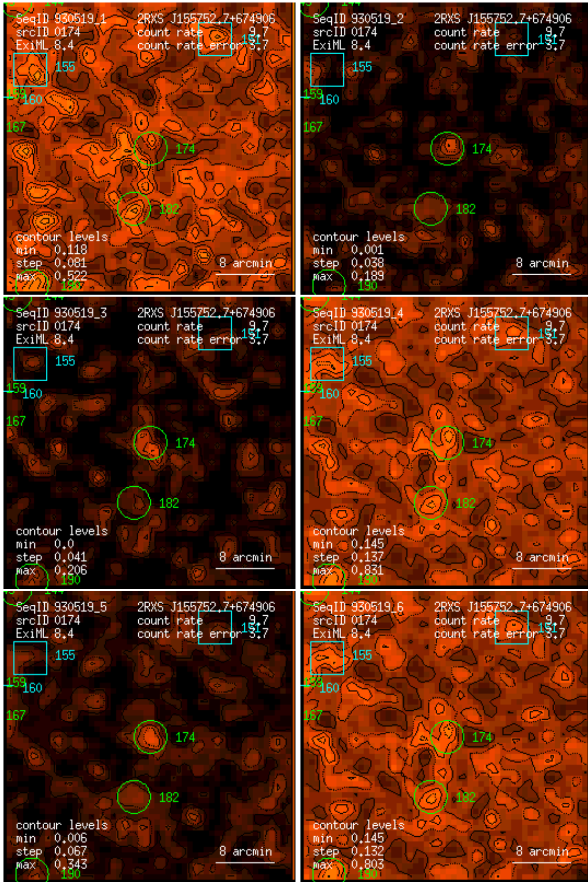
Figure 174: RASS 930519: detection 0174: band rate images, Gaussian filter: (1) PSPC channels 11 – 41, (2) 52 – 90, (3) 91 – 201, (4) 11 – 235, (5) 52 – 201, (6) 11 – 201. Broad band rates in counts/ks. Band rate contour levels in counts/ks/arcmin 2 .
