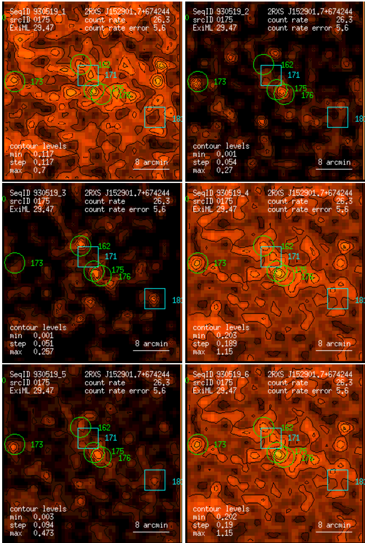
Figure 175: RASS 930519: detection 0175: band rate images, Gaussian filter: (1) PSPC channels 11 – 41, (2) 52 – 90, (3) 91 – 201, (4) 11 – 235, (5) 52 – 201, (6) 11 – 201. Broad band rates in counts/ks. Band rate contour levels in counts/ks/arcmin 2 .
