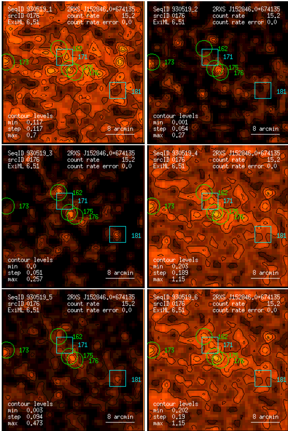
Figure 176: RASS 930519: detection 0176: band rate images, Gaussian filter: (1) PSPC channels 11 – 41, (2) 52 – 90, (3) 91 – 201, (4) 11 – 235, (5) 52 – 201, (6) 11 – 201. Broad band rates in counts/ks. Band rate contour levels in counts/ks/arcmin 2 .
