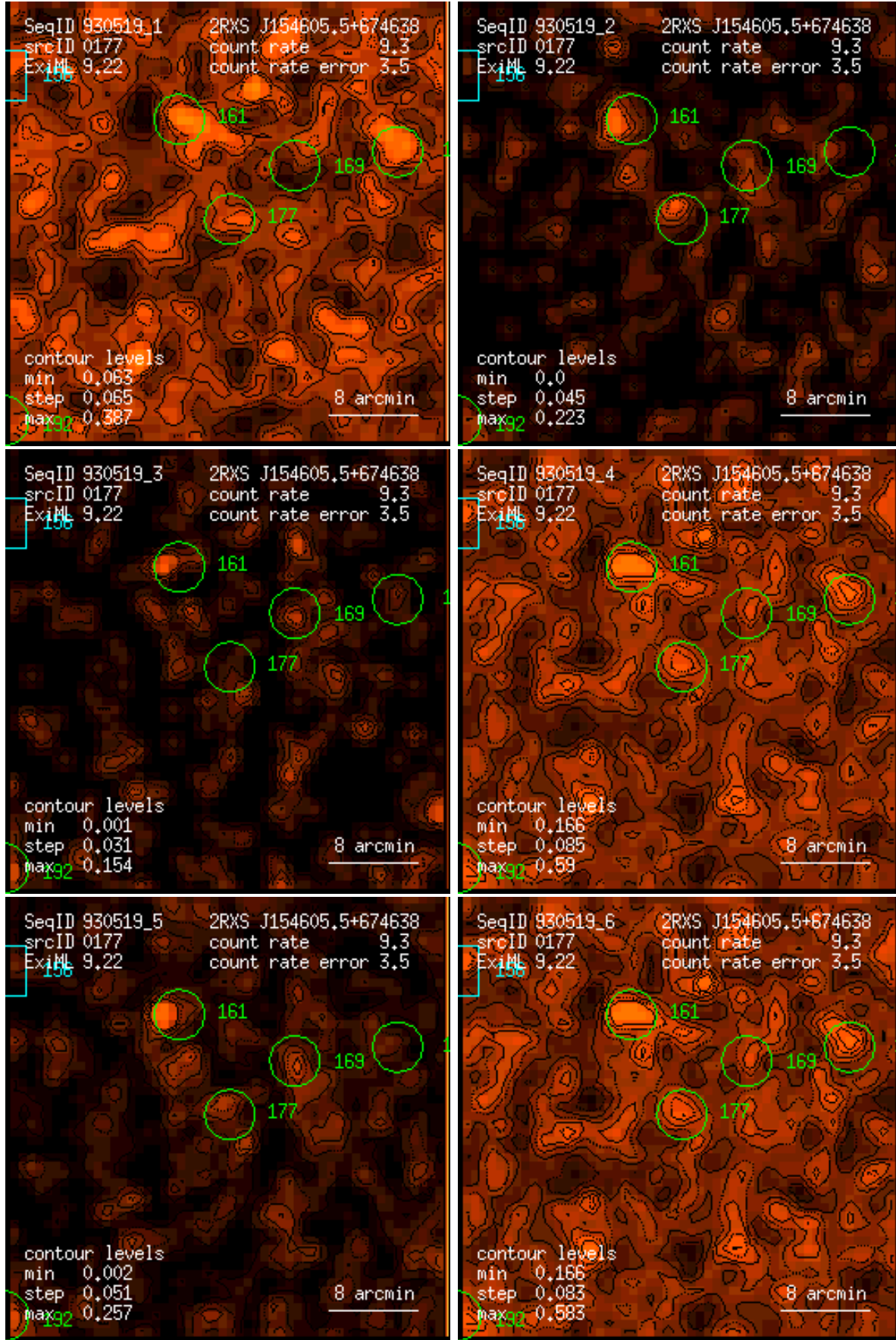
Figure 177: RASS 930519: detection 0177: band rate images, Gaussian filter: (1) PSPC channels 11 – 41, (2) 52 – 90, (3) 91 – 201, (4) 11 – 235, (5) 52 – 201, (6) 11 – 201. Broad band rates in counts/ks. Band rate contour levels in counts/ks/arcmin 2 .
