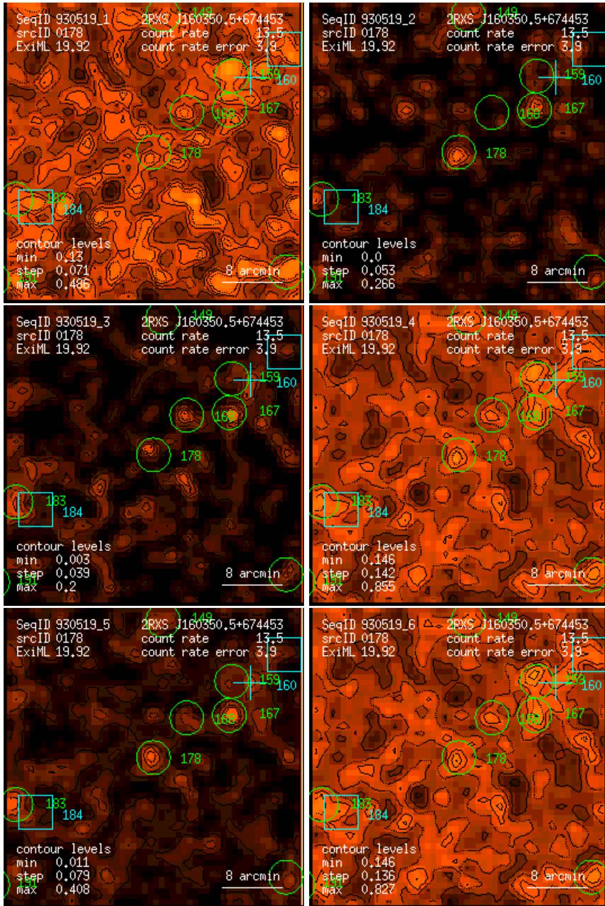
Figure 178: RASS 930519: detection 0178: band rate images, Gaussian filter: (1) PSPC channels 11 – 41, (2) 52 – 90, (3) 91 – 201, (4) 11 – 235, (5) 52 – 201, (6) 11 – 201. Broad band rates in counts/ks. Band rate contour levels in counts/ks/arcmin 2 .
