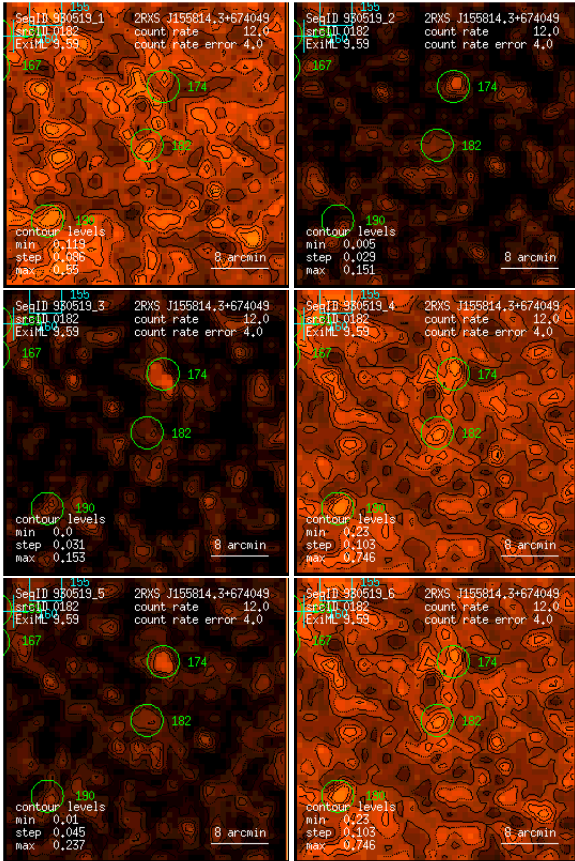
Figure 182: RASS 930519: detection 0182: band rate images, Gaussian filter: (1) PSPC channels 11 – 41, (2) 52 – 90, (3) 91 – 201, (4) 11 – 235, (5) 52 – 201, (6) 11 – 201. Broad band rates in counts/ks. Band rate contour levels in counts/ks/arcmin 2 .
