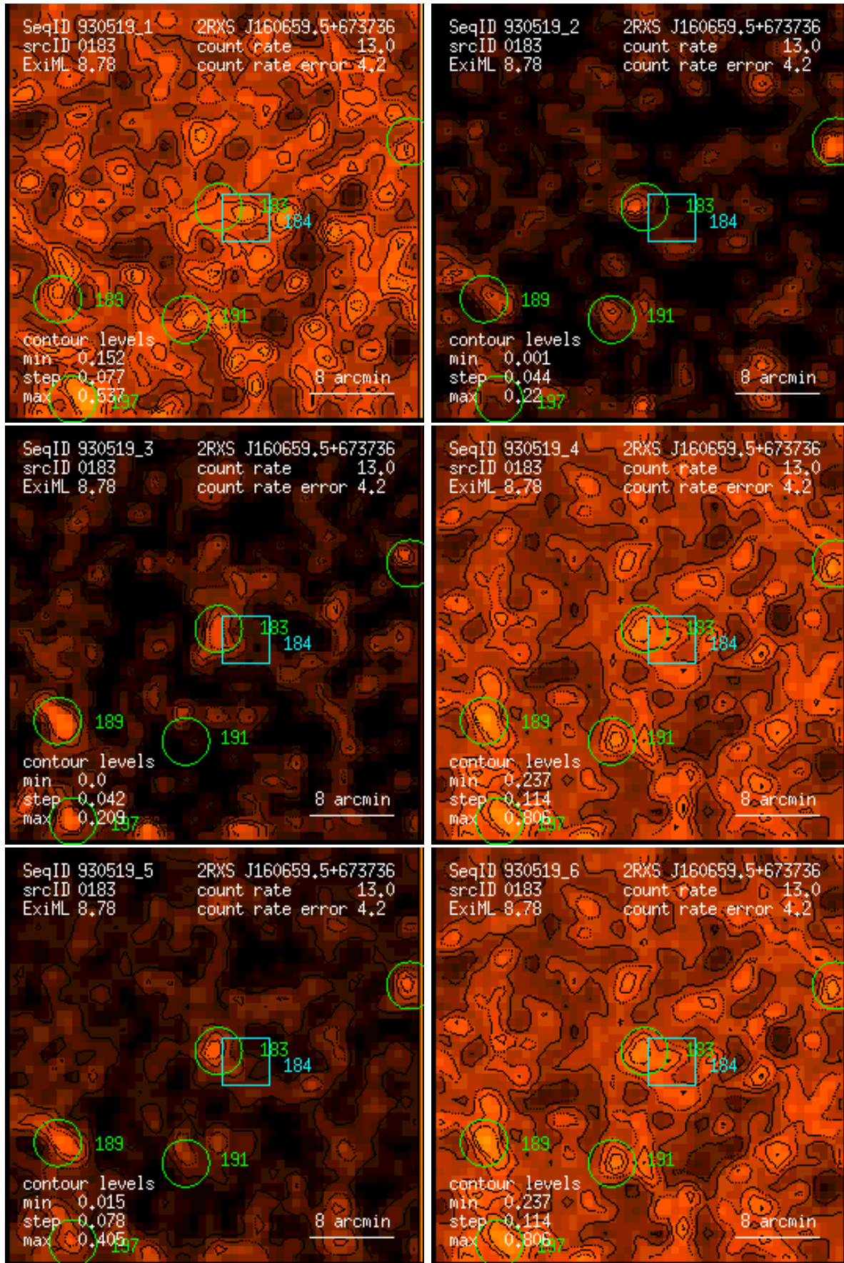
Figure 183: RASS 930519: detection 0183: band rate images, Gaussian filter: (1) PSPC channels 11 – 41, (2) 52 – 90, (3) 91 – 201, (4) 11 – 235, (5) 52 – 201, (6) 11 – 201. Broad band rates in counts/ks. Band rate contour levels in counts/ks/arcmin 2 .
