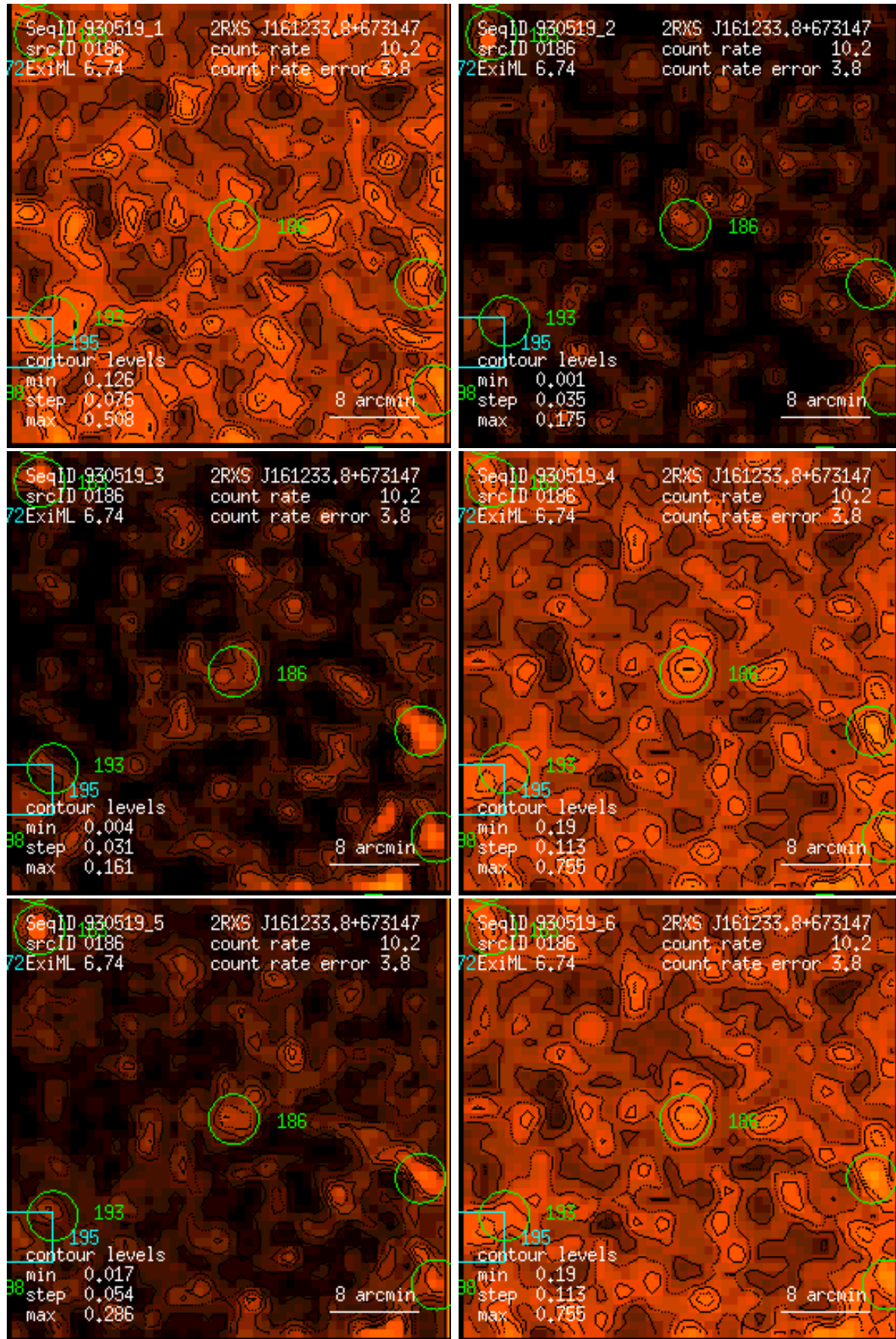
Figure 186: RASS 930519: detection 0186: band rate images, Gaussian filter: (1) PSPC channels 11 – 41, (2) 52 – 90, (3) 91 – 201, (4) 11 – 235, (5) 52 – 201, (6) 11 – 201. Broad band rates in counts/ks. Band rate contour levels in counts/ks/arcmin 2 .
