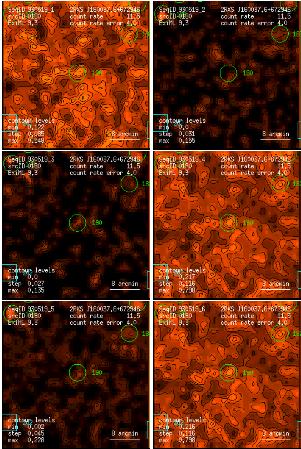
Figure 190: RASS 930519: detection 0190: band rate images, Gaussian filter: (1) PSPC channels 11 – 41, (2) 52 – 90, (3) 91 – 201, (4) 11 – 235, (5) 52 – 201, (6) 11 – 201. Broad band rates in counts/ks. Band rate contour levels in counts/ks/arcmin 2 .
