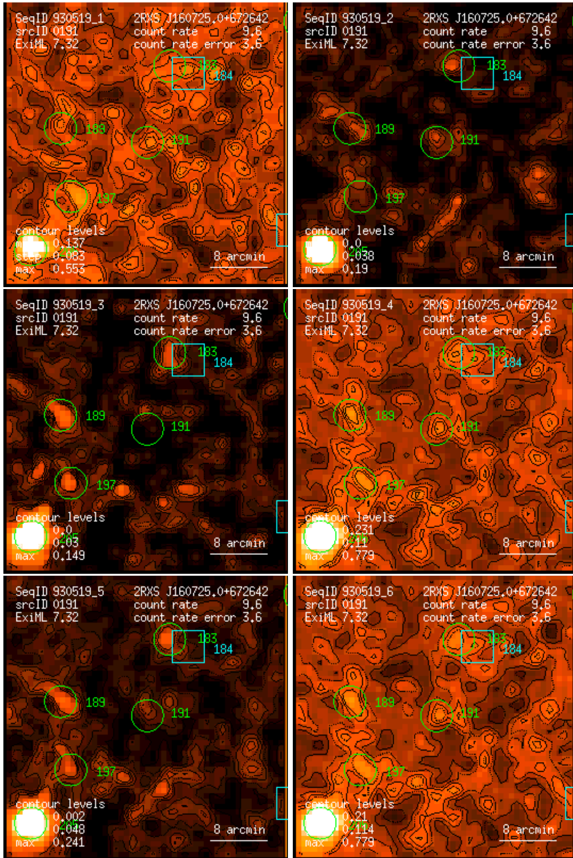
Figure 191: RASS 930519: detection 0191: band rate images, Gaussian filter: (1) PSPC channels 11 – 41, (2) 52 – 90, (3) 91 – 201, (4) 11 – 235, (5) 52 – 201, (6) 11 – 201. Broad band rates in counts/ks. Band rate contour levels in counts/ks/arcmin 2 .
