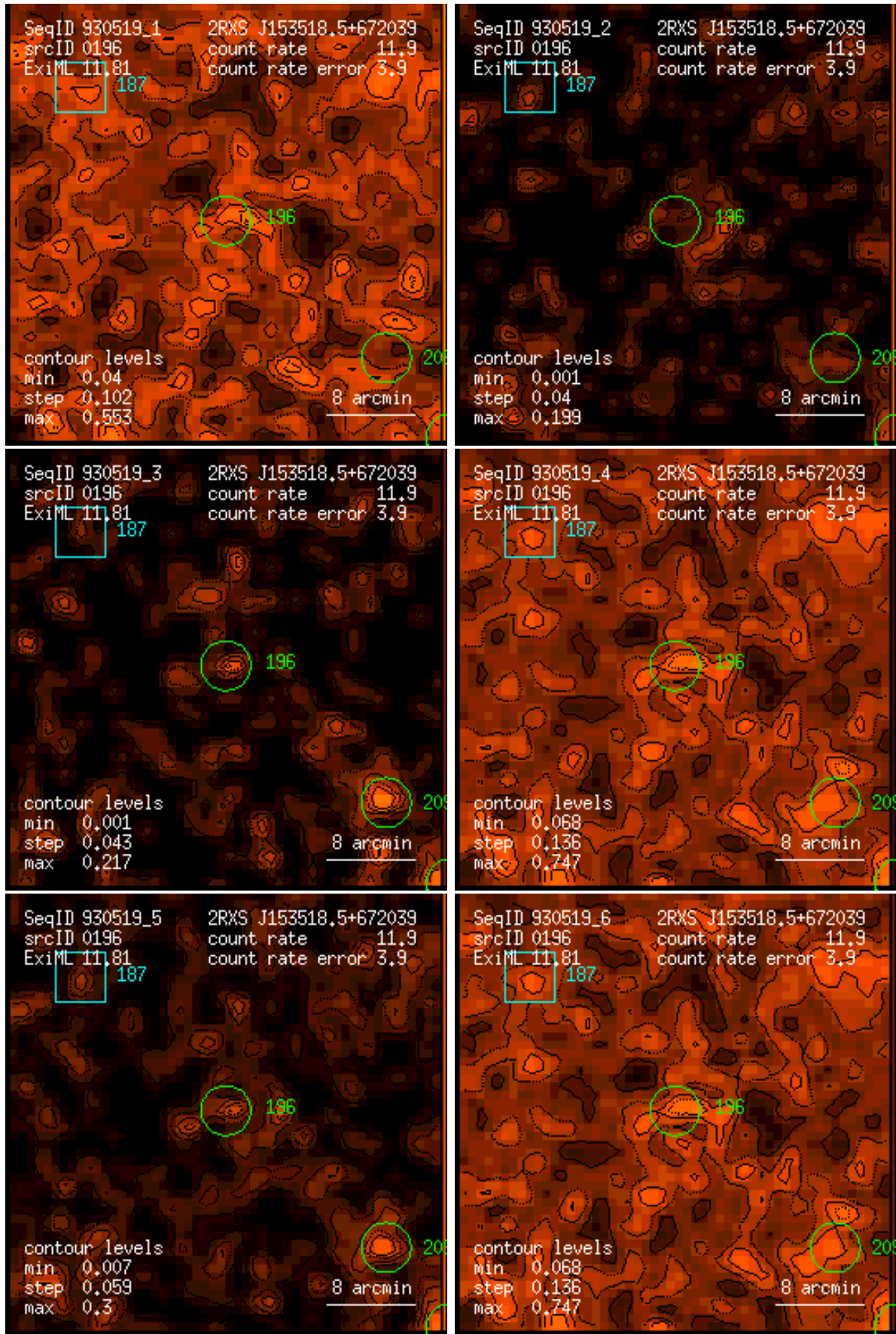
Figure 196: RASS 930519: detection 0196: band rate images, Gaussian filter: (1) PSPC channels 11 – 41, (2) 52 – 90, (3) 91 – 201, (4) 11 – 235, (5) 52 – 201, (6) 11 – 201. Broad band rates in counts/ks. Band rate contour levels in counts/ks/arcmin 2 .
