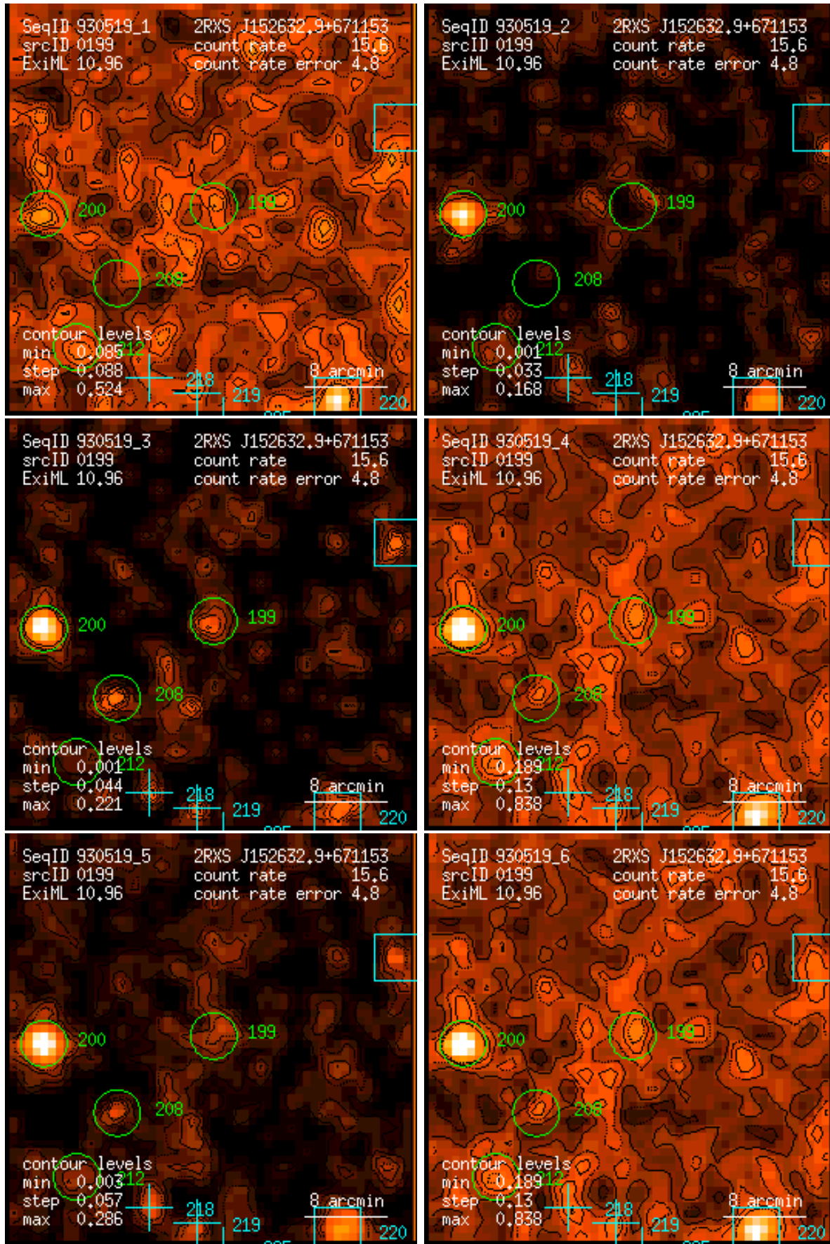
Figure 199: RASS 930519: detection 0199: band rate images, Gaussian filter: (1) PSPC channels 11 – 41, (2) 52 – 90, (3) 91 – 201, (4) 11 – 235, (5) 52 – 201, (6) 11 – 201. Broad band rates in counts/ks. Band rate contour levels in counts/ks/arcmin 2 .
