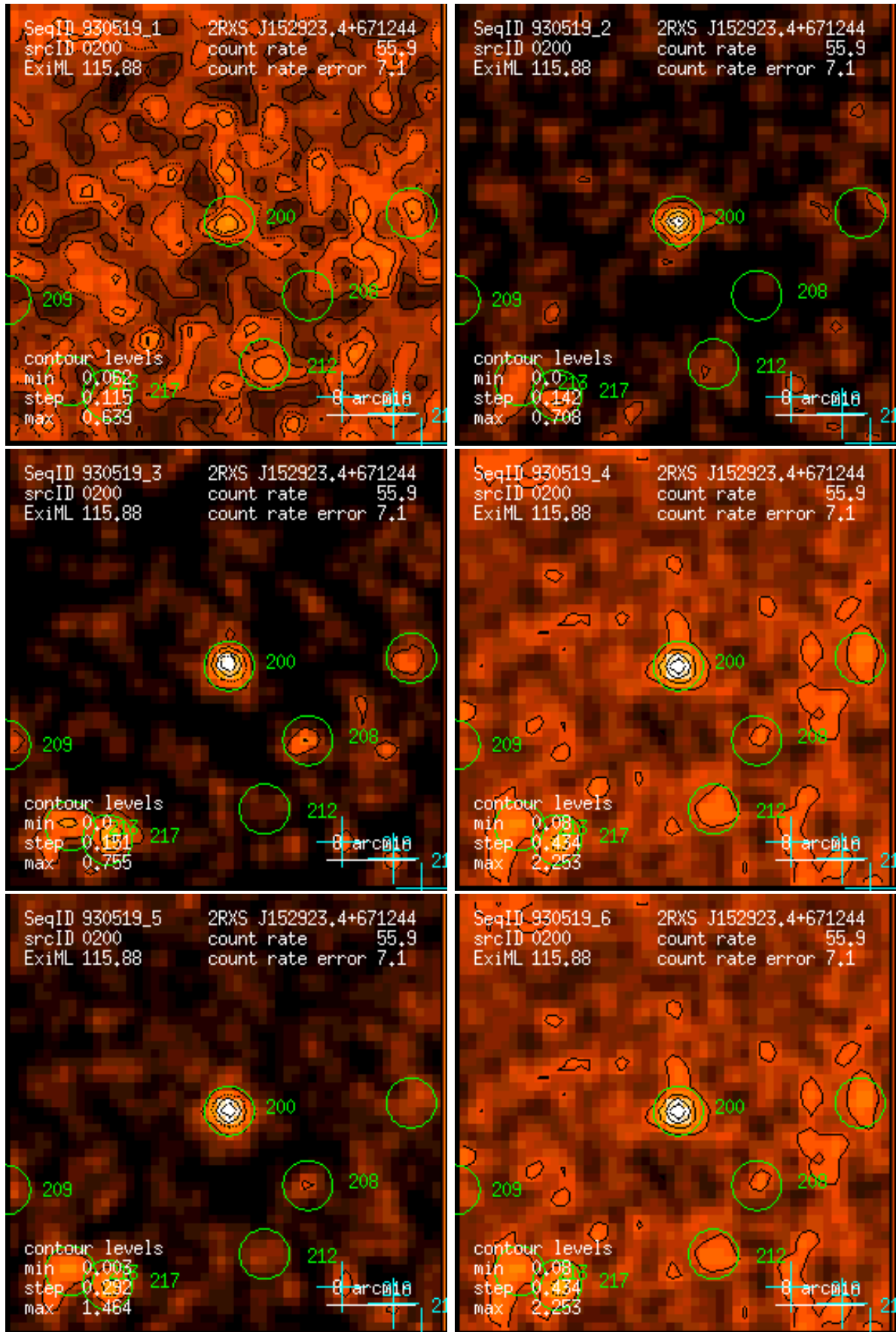
Figure 200: RASS 930519: detection 0200: band rate images, Gaussian filter: (1) PSPC channels 11 – 41, (2) 52 – 90, (3) 91 – 201, (4) 11 – 235, (5) 52 – 201, (6) 11 – 201. Broad band rates in counts/ks. Band rate contour levels in counts/ks/arcmin 2 .
