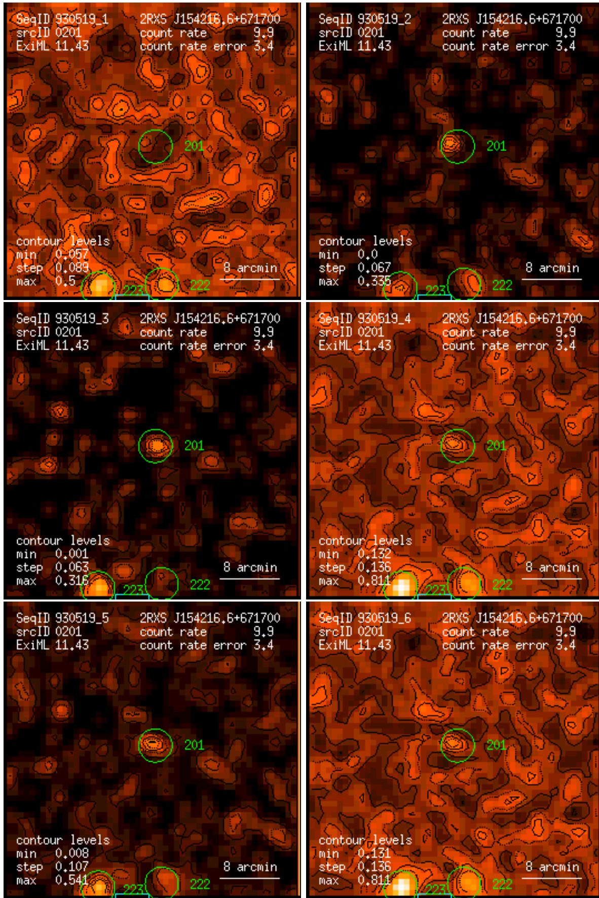
Figure 201: RASS 930519: detection 0201: band rate images, Gaussian filter: (1) PSPC channels 11 – 41, (2) 52 – 90, (3) 91 – 201, (4) 11 – 235, (5) 52 – 201, (6) 11 – 201. Broad band rates in counts/ks. Band rate contour levels in counts/ks/arcmin 2 .
