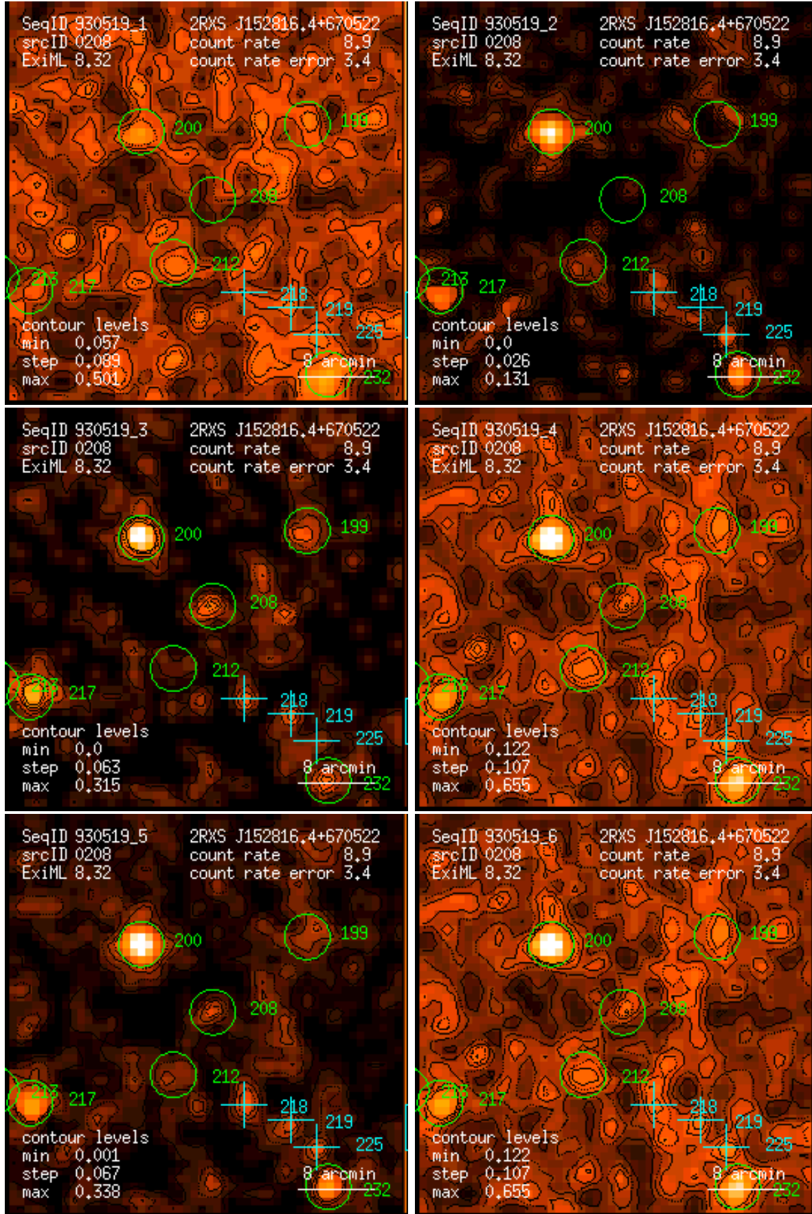
Figure 208: RASS 930519: detection 0208: band rate images, Gaussian filter: (1) PSPC channels 11 – 41, (2) 52 – 90, (3) 91 – 201, (4) 11 – 235, (5) 52 – 201, (6) 11 – 201. Broad band rates in counts/ks. Band rate contour levels in counts/ks/arcmin 2 .
