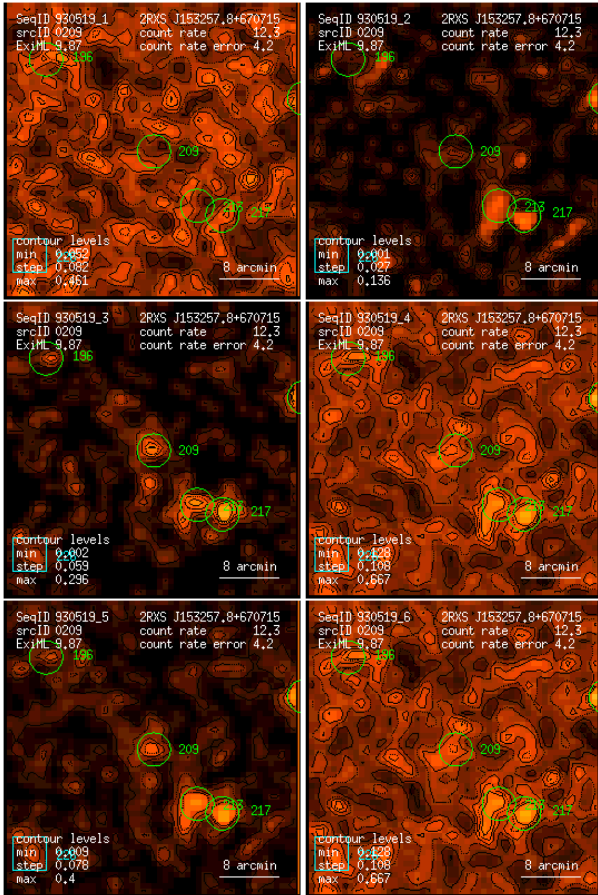
Figure 209: RASS 930519: detection 0209: band rate images, Gaussian filter: (1) PSPC channels 11 – 41, (2) 52 – 90, (3) 91 – 201, (4) 11 – 235, (5) 52 – 201, (6) 11 – 201. Broad band rates in counts/ks. Band rate contour levels in counts/ks/arcmin 2 .
