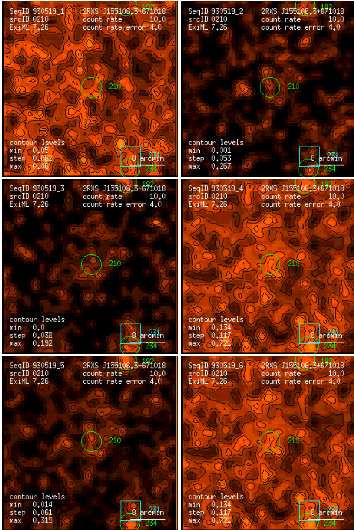
Figure 210: RASS 930519: detection 0210: band rate images, Gaussian filter: (1) PSPC channels 11 – 41, (2) 52 – 90, (3) 91 – 201, (4) 11 – 235, (5) 52 – 201, (6) 11 – 201. Broad band rates in counts/ks. Band rate contour levels in counts/ks/arcmin 2 .
