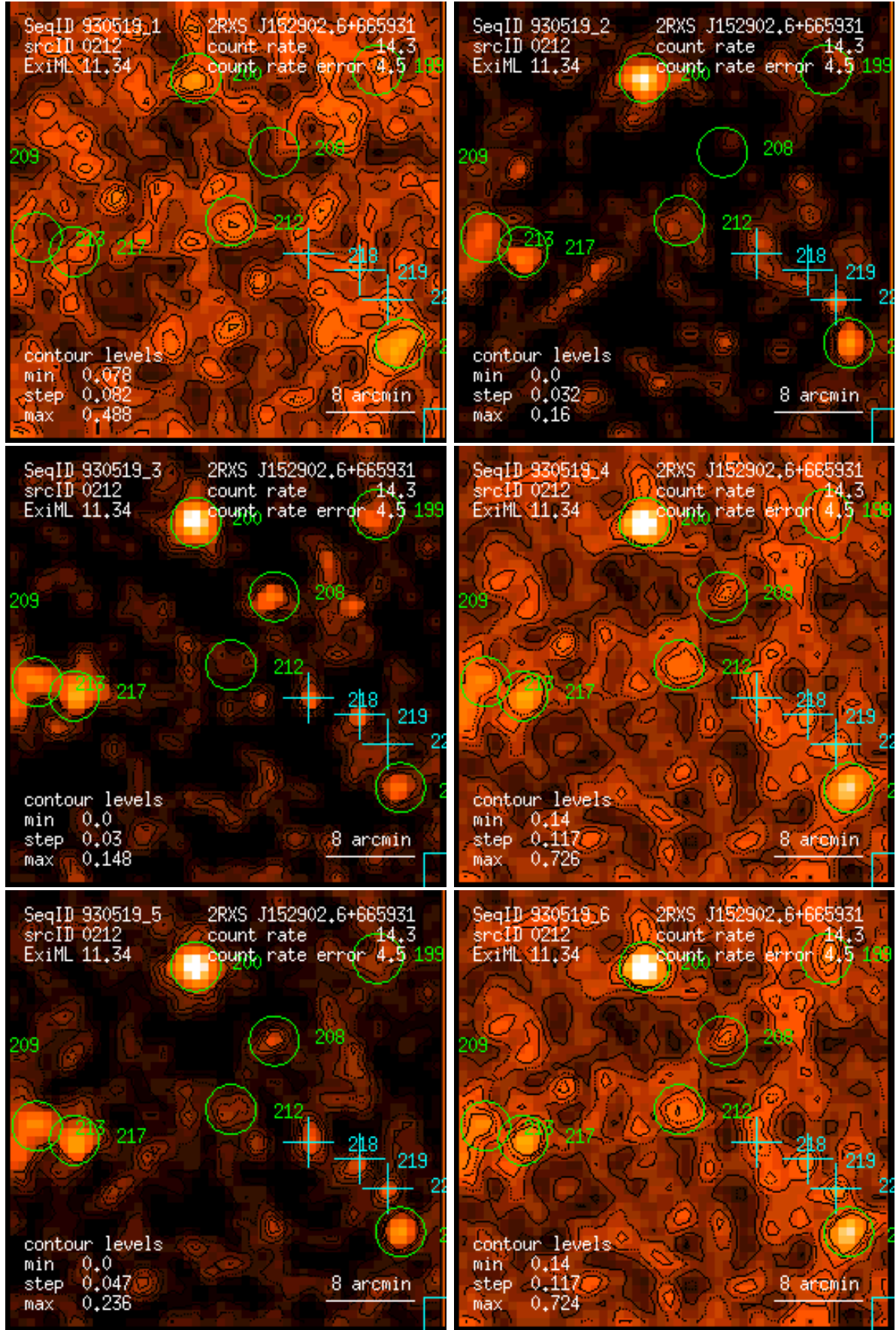
Figure 212: RASS 930519: detection 0212: band rate images, Gaussian filter: (1) PSPC channels 11 – 41, (2) 52 – 90, (3) 91 – 201, (4) 11 – 235, (5) 52 – 201, (6) 11 – 201. Broad band rates in counts/ks. Band rate contour levels in counts/ks/arcmin 2 .
