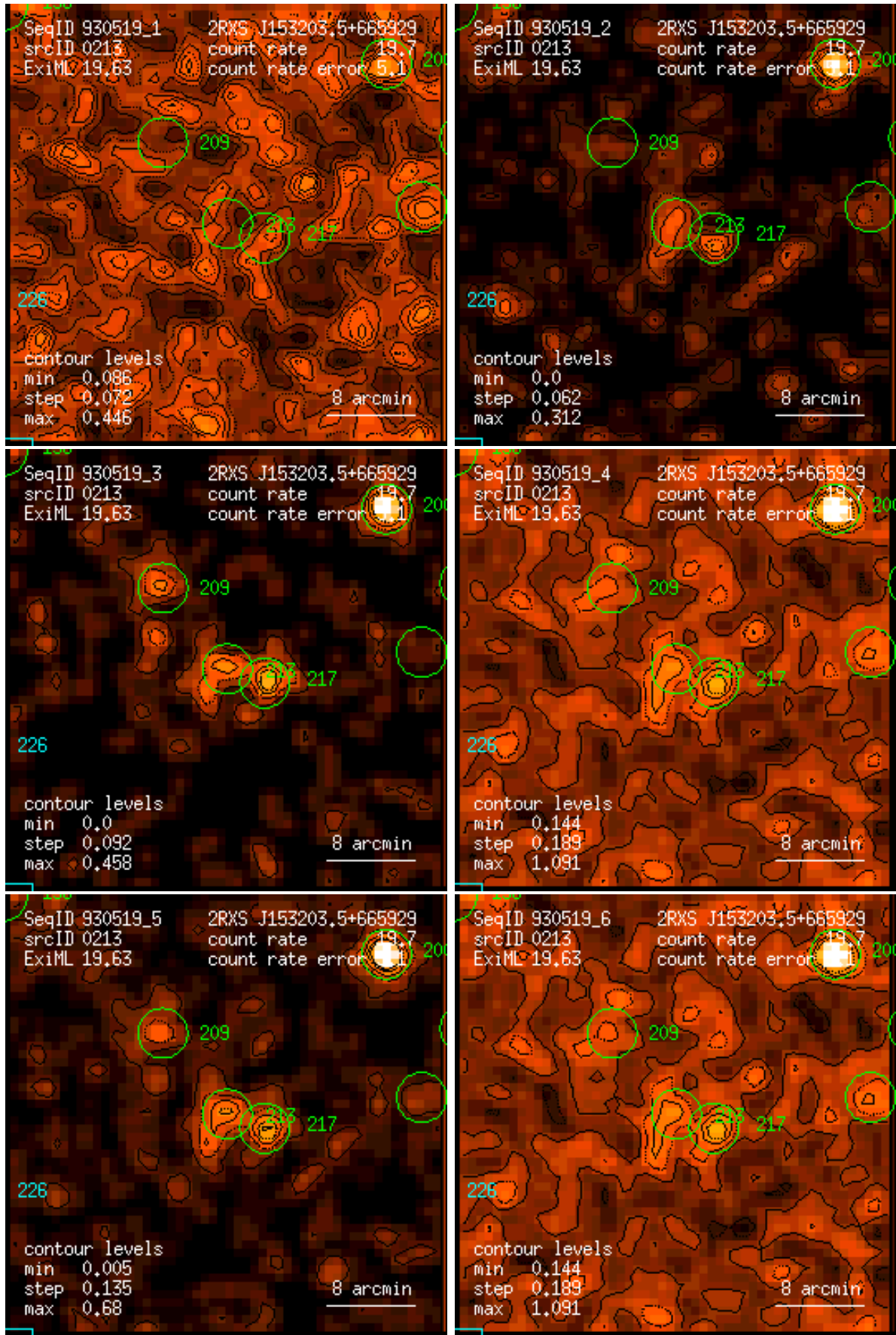
Figure 213: RASS 930519: detection 0213: band rate images, Gaussian filter: (1) PSPC channels 11 – 41, (2) 52 – 90, (3) 91 – 201, (4) 11 – 235, (5) 52 – 201, (6) 11 – 201. Broad band rates in counts/ks. Band rate contour levels in counts/ks/arcmin 2 .
