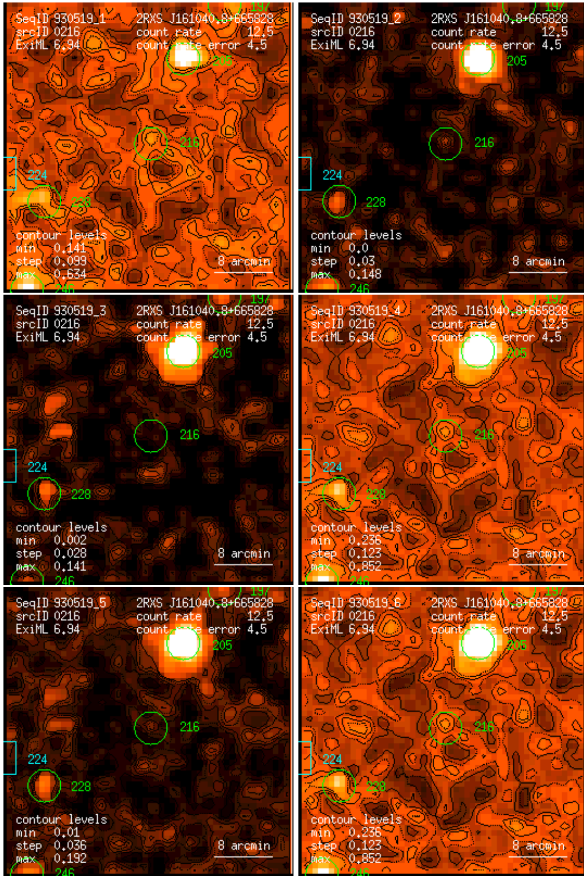
Figure 216: RASS 930519: detection 0216: band rate images, Gaussian filter: (1) PSPC channels 11 – 41, (2) 52 – 90, (3) 91 – 201, (4) 11 – 235, (5) 52 – 201, (6) 11 – 201. Broad band rates in counts/ks. Band rate contour levels in counts/ks/arcmin 2 .
