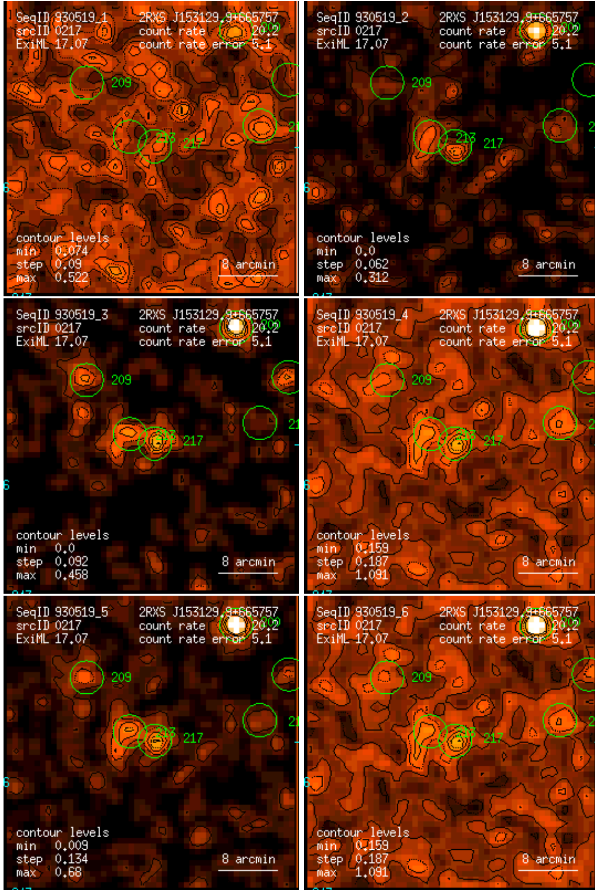
Figure 217: RASS 930519: detection 0217: band rate images, Gaussian filter: (1) PSPC channels 11 – 41, (2) 52 – 90, (3) 91 – 201, (4) 11 – 235, (5) 52 – 201, (6) 11 – 201. Broad band rates in counts/ks. Band rate contour levels in counts/ks/arcmin 2 .
