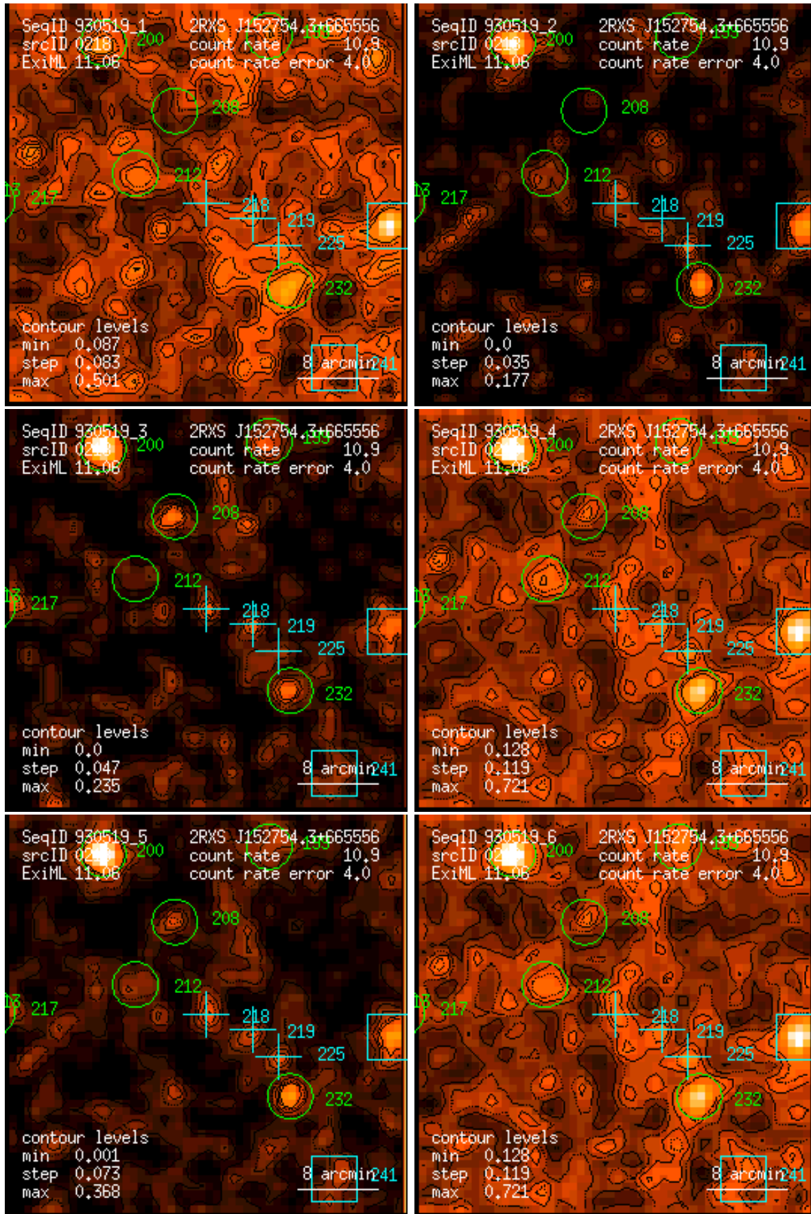
Figure 218: RASS 930519: detection 0218: band rate images, Gaussian filter: (1) PSPC channels 11 – 41, (2) 52 – 90, (3) 91 – 201, (4) 11 – 235, (5) 52 – 201, (6) 11 – 201. Broad band rates in counts/ks. Band rate contour levels in counts/ks/arcmin 2 .
