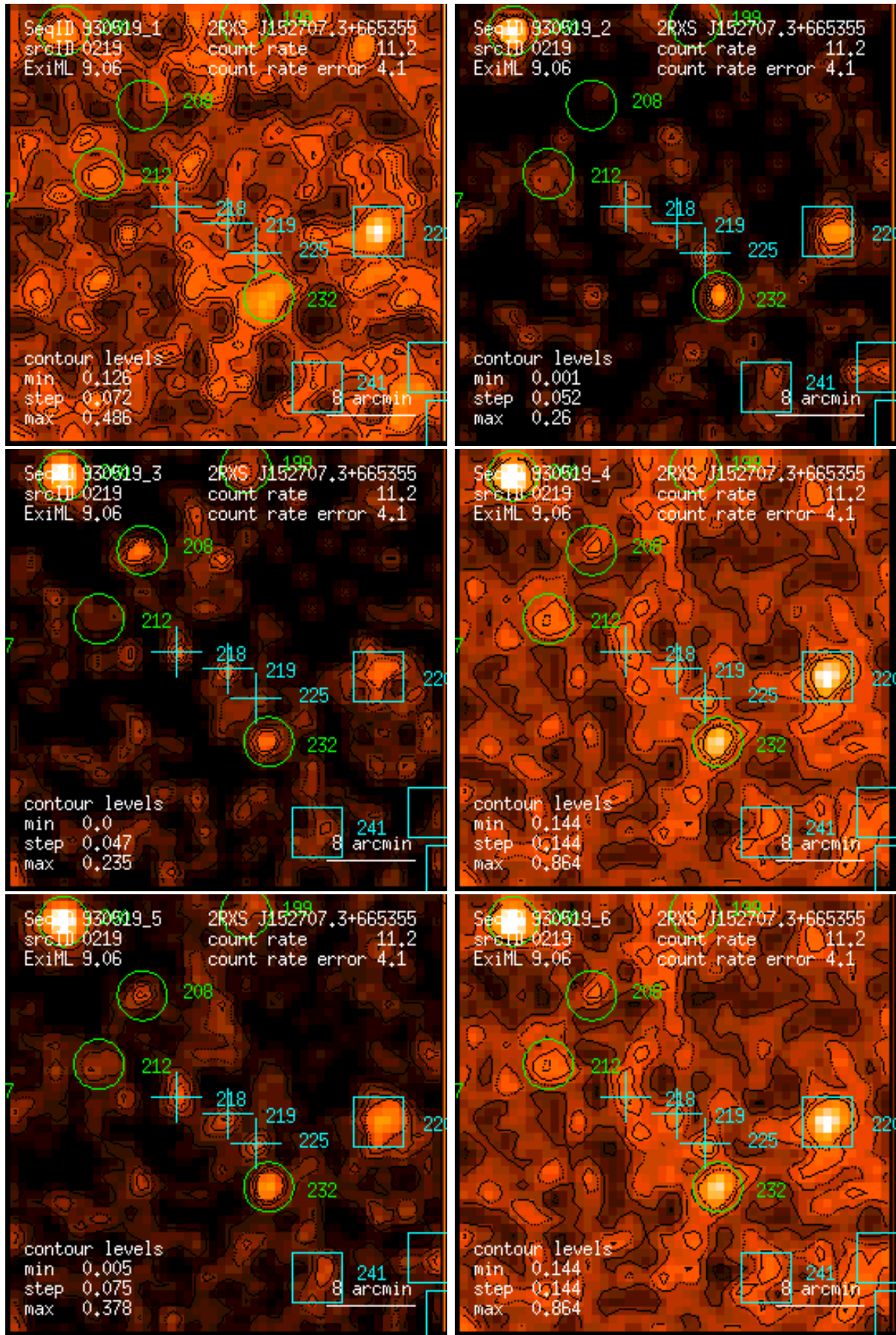
Figure 219: RASS 930519: detection 0219: band rate images, Gaussian filter: (1) PSPC channels 11 – 41, (2) 52 – 90, (3) 91 – 201, (4) 11 – 235, (5) 52 – 201, (6) 11 – 201. Broad band rates in counts/ks. Band rate contour levels in counts/ks/arcmin 2 .
