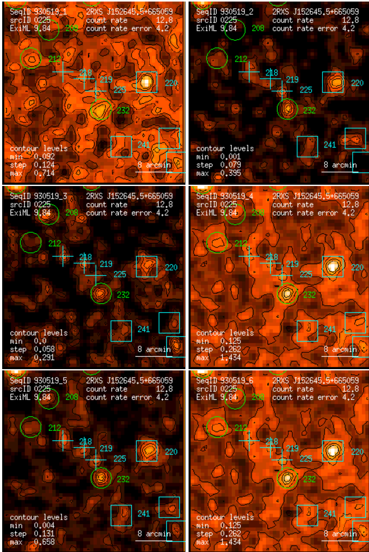
Figure 225: RASS 930519: detection 0225: band rate images, Gaussian filter: (1) PSPC channels 11 – 41, (2) 52 – 90, (3) 91 – 201, (4) 11 – 235, (5) 52 – 201, (6) 11 – 201. Broad band rates in counts/ks. Band rate contour levels in counts/ks/arcmin 2 .
