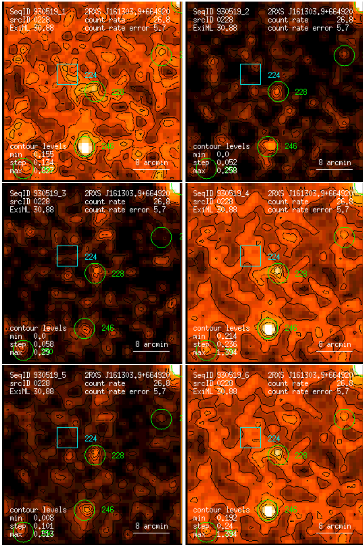
Figure 228: RASS 930519: detection 0228: band rate images, Gaussian filter: (1) PSPC channels 11 – 41, (2) 52 – 90, (3) 91 – 201, (4) 11 – 235, (5) 52 – 201, (6) 11 – 201. Broad band rates in counts/ks. Band rate contour levels in counts/ks/arcmin 2 .
