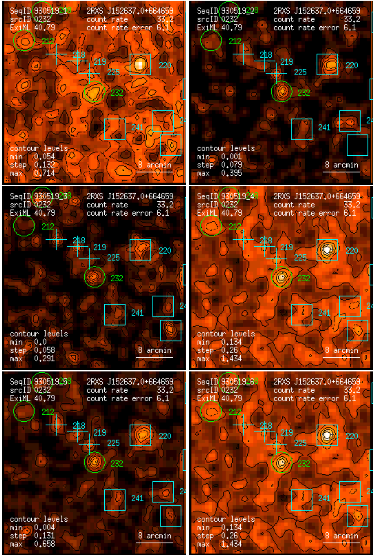
Figure 232: RASS 930519: detection 0232: band rate images, Gaussian filter: (1) PSPC channels 11 – 41, (2) 52 – 90, (3) 91 – 201, (4) 11 – 235, (5) 52 – 201, (6) 11 – 201. Broad band rates in counts/ks. Band rate contour levels in counts/ks/arcmin 2 .
