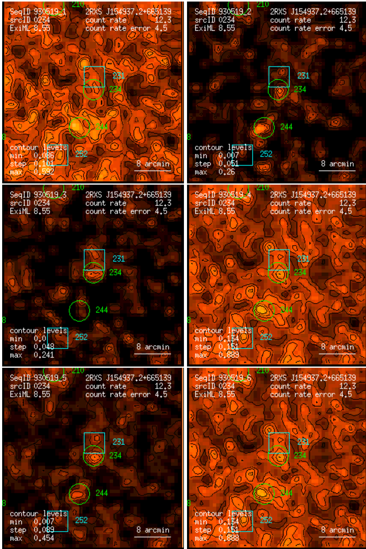
Figure 234: RASS 930519: detection 0234: band rate images, Gaussian filter: (1) PSPC channels 11 – 41, (2) 52 – 90, (3) 91 – 201, (4) 11 – 235, (5) 52 – 201, (6) 11 – 201. Broad band rates in counts/ks. Band rate contour levels in counts/ks/arcmin 2 .
