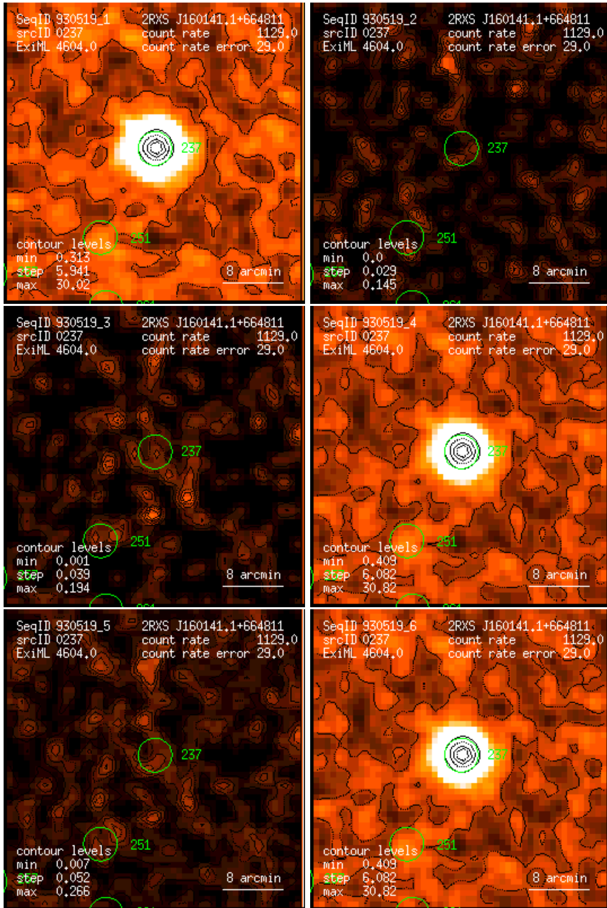
Figure 237: RASS 930519: detection 0237: band rate images, Gaussian filter: (1) PSPC channels 11 – 41, (2) 52 – 90, (3) 91 – 201, (4) 11 – 235, (5) 52 – 201, (6) 11 – 201. Broad band rates in counts/ks. Band rate contour levels in counts/ks/arcmin 2 .
