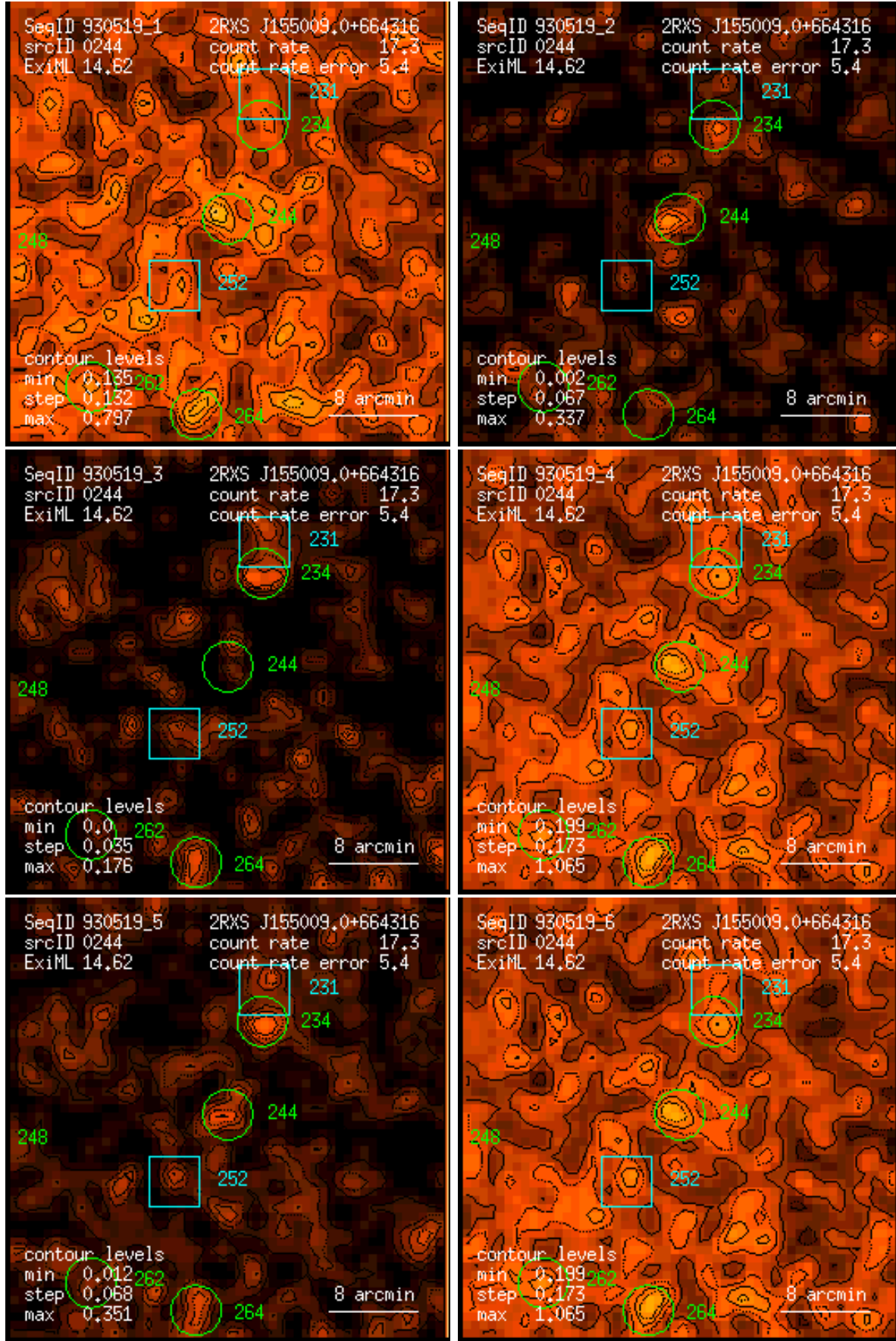
Figure 244: RASS 930519: detection 0244: band rate images, Gaussian filter: (1) PSPC channels 11 – 41, (2) 52 – 90, (3) 91 – 201, (4) 11 – 235, (5) 52 – 201, (6) 11 – 201. Broad band rates in counts/ks. Band rate contour levels in counts/ks/arcmin 2 .
