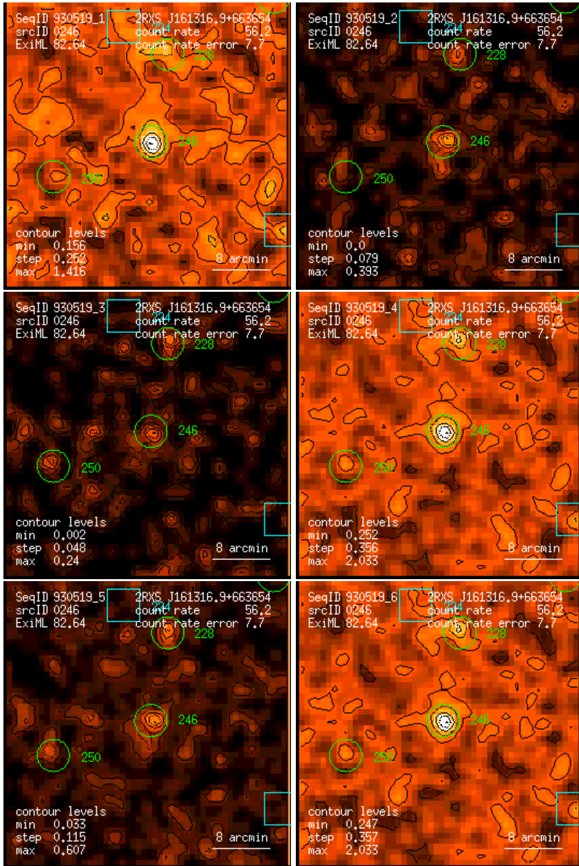
Figure 246: RASS 930519: detection 0246: band rate images, Gaussian filter: (1) PSPC channels 11 – 41, (2) 52 – 90, (3) 91 – 201, (4) 11 – 235, (5) 52 – 201, (6) 11 – 201. Broad band rates in counts/ks. Band rate contour levels in counts/ks/arcmin 2 .
