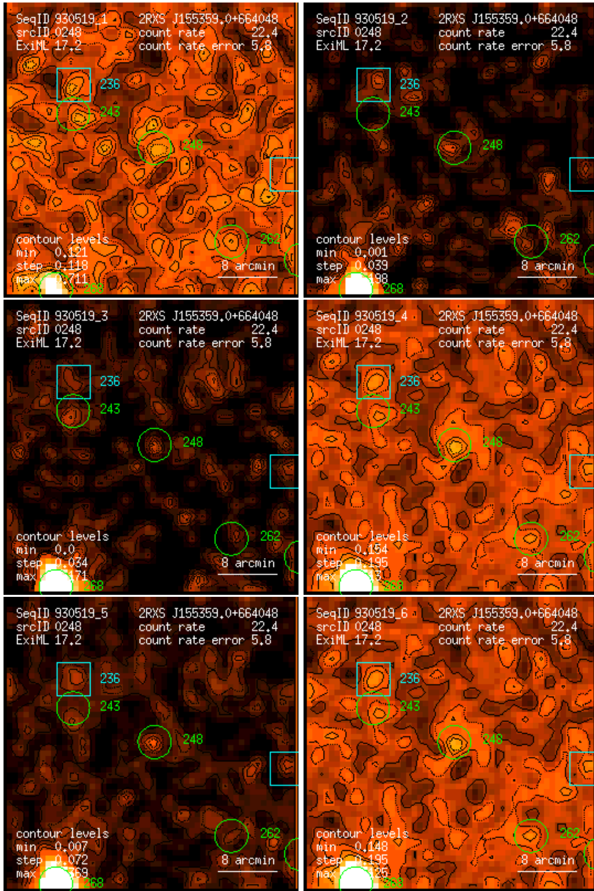
Figure 248: RASS 930519: detection 0248: band rate images, Gaussian filter: (1) PSPC channels 11 – 41, (2) 52 – 90, (3) 91 – 201, (4) 11 – 235, (5) 52 – 201, (6) 11 – 201. Broad band rates in counts/ks. Band rate contour levels in counts/ks/arcmin 2 .
