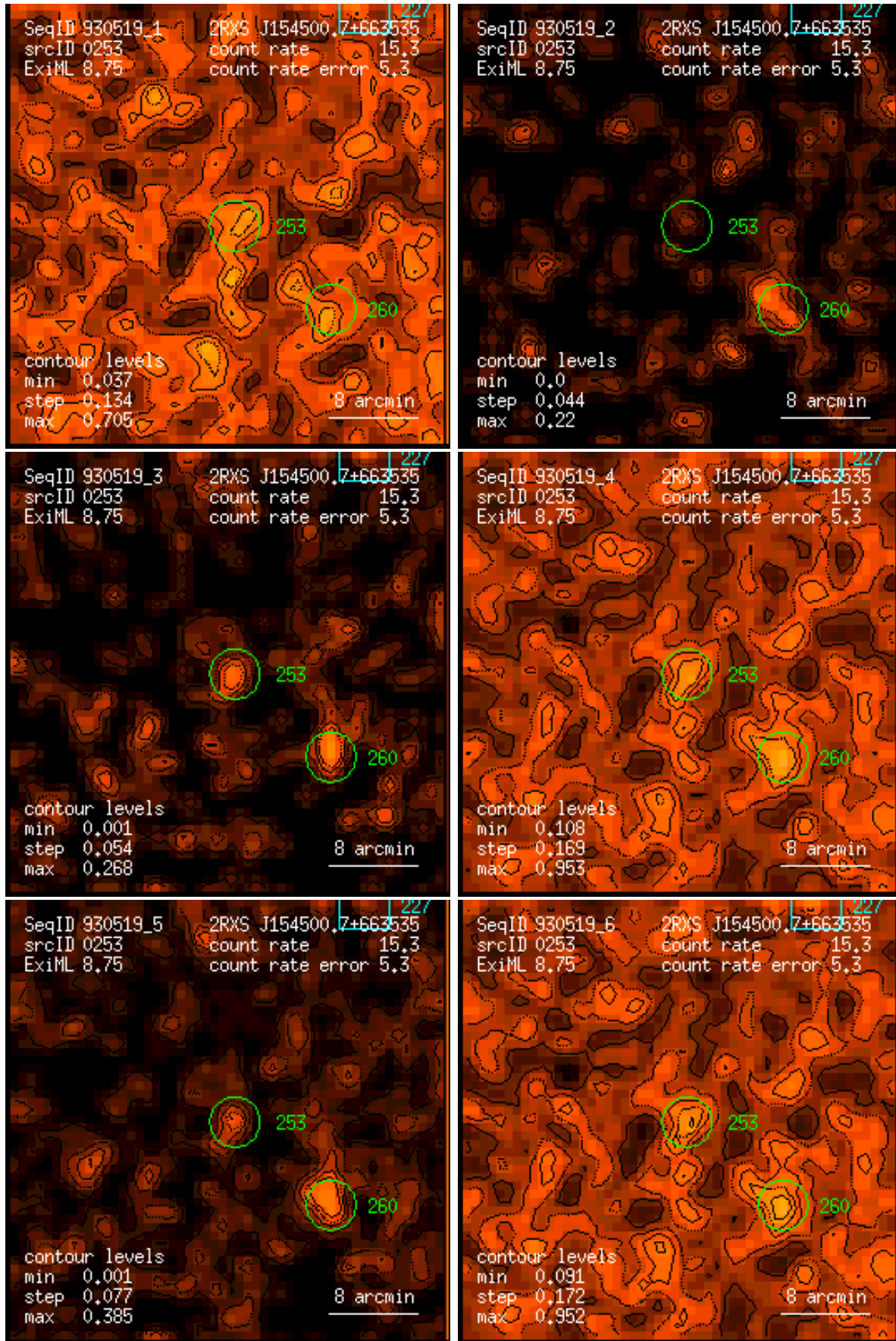
Figure 253: RASS 930519: detection 0253: band rate images, Gaussian filter: (1) PSPC channels 11 – 41, (2) 52 – 90, (3) 91 – 201, (4) 11 – 235, (5) 52 – 201, (6) 11 – 201. Broad band rates in counts/ks. Band rate contour levels in counts/ks/arcmin 2 .
