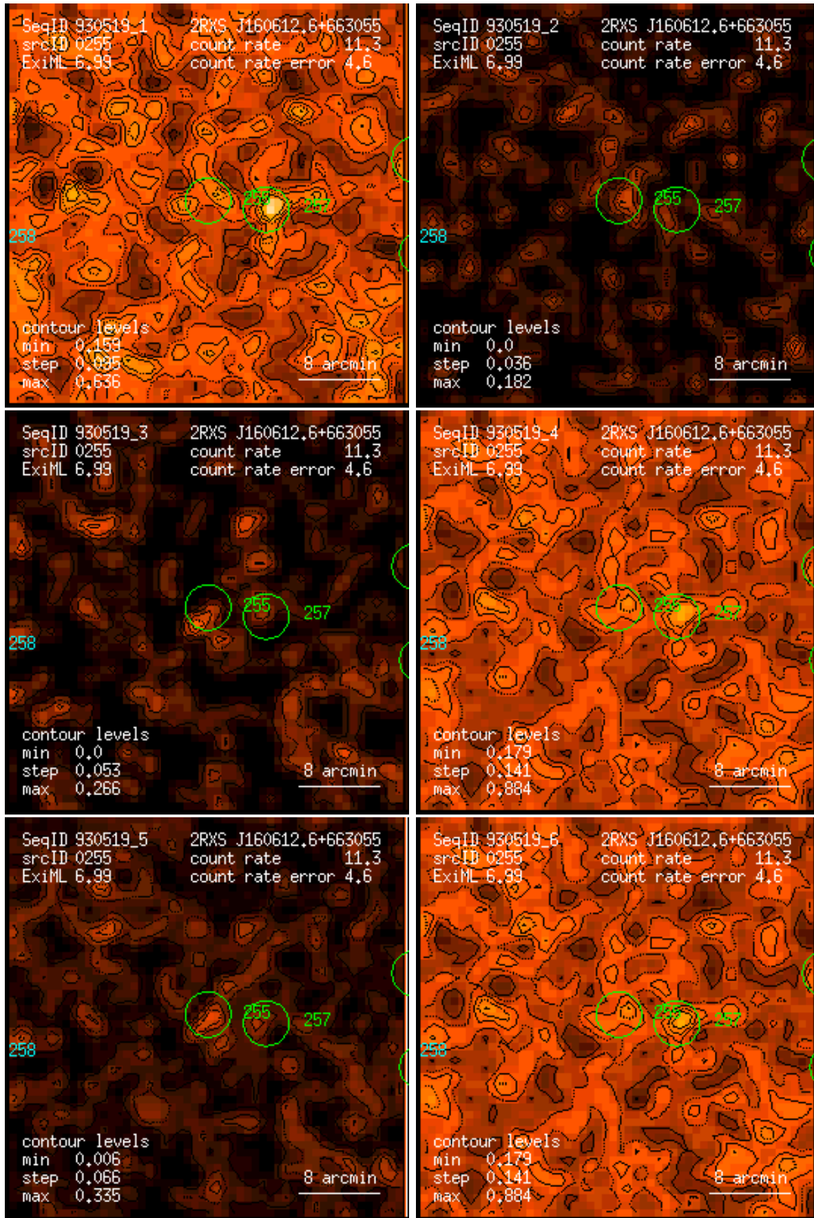
Figure 255: RASS 930519: detection 0255: band rate images, Gaussian filter: (1) PSPC channels 11 – 41, (2) 52 – 90, (3) 91 – 201, (4) 11 – 235, (5) 52 – 201, (6) 11 – 201. Broad band rates in counts/ks. Band rate contour levels in counts/ks/arcmin 2 .
