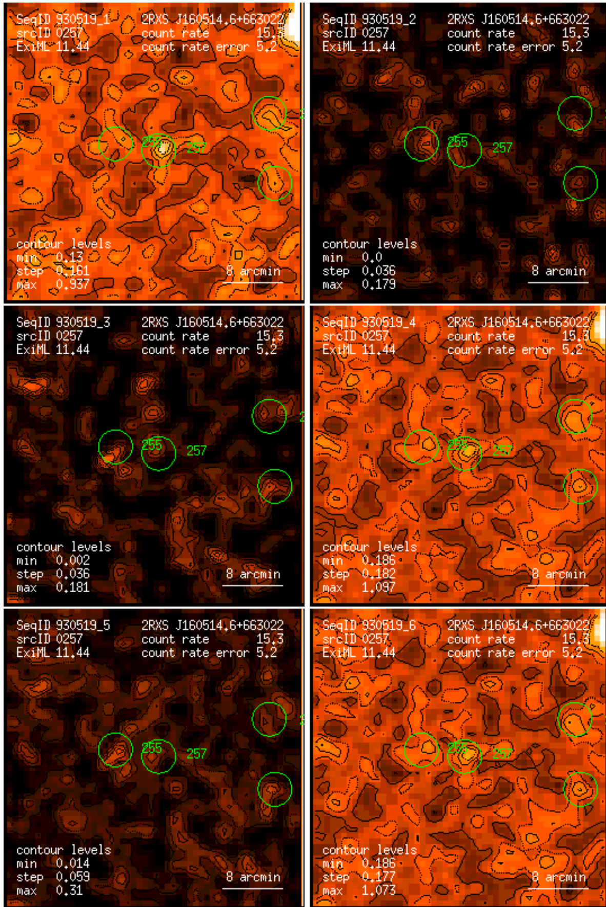
Figure 257: RASS 930519: detection 0257: band rate images, Gaussian filter: (1) PSPC channels 11 – 41, (2) 52 – 90, (3) 91 – 201, (4) 11 – 235, (5) 52 – 201, (6) 11 – 201. Broad band rates in counts/ks. Band rate contour levels in counts/ks/arcmin 2 .
