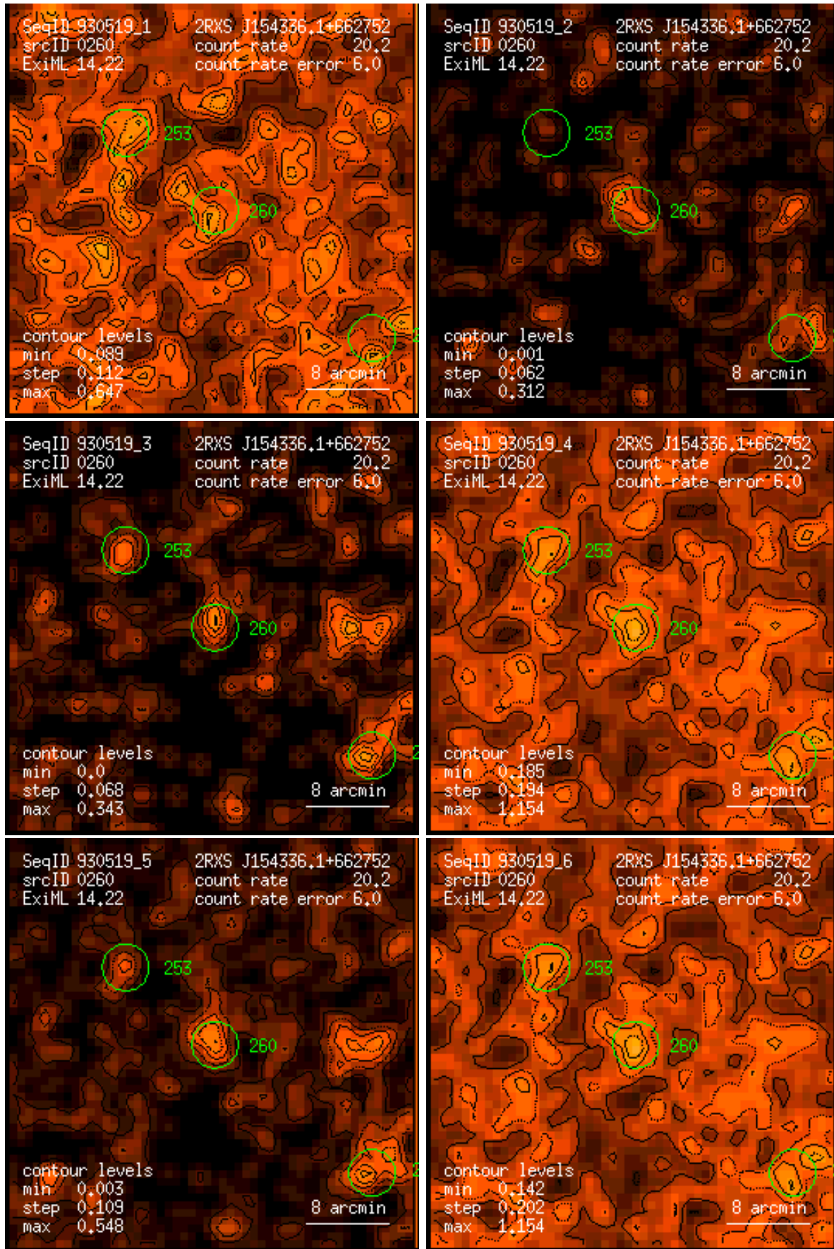
Figure 260: RASS 930519: detection 0260: band rate images, Gaussian filter: (1) PSPC channels 11 – 41, (2) 52 – 90, (3) 91 – 201, (4) 11 – 235, (5) 52 – 201, (6) 11 – 201. Broad band rates in counts/ks. Band rate contour levels in counts/ks/arcmin 2 .
