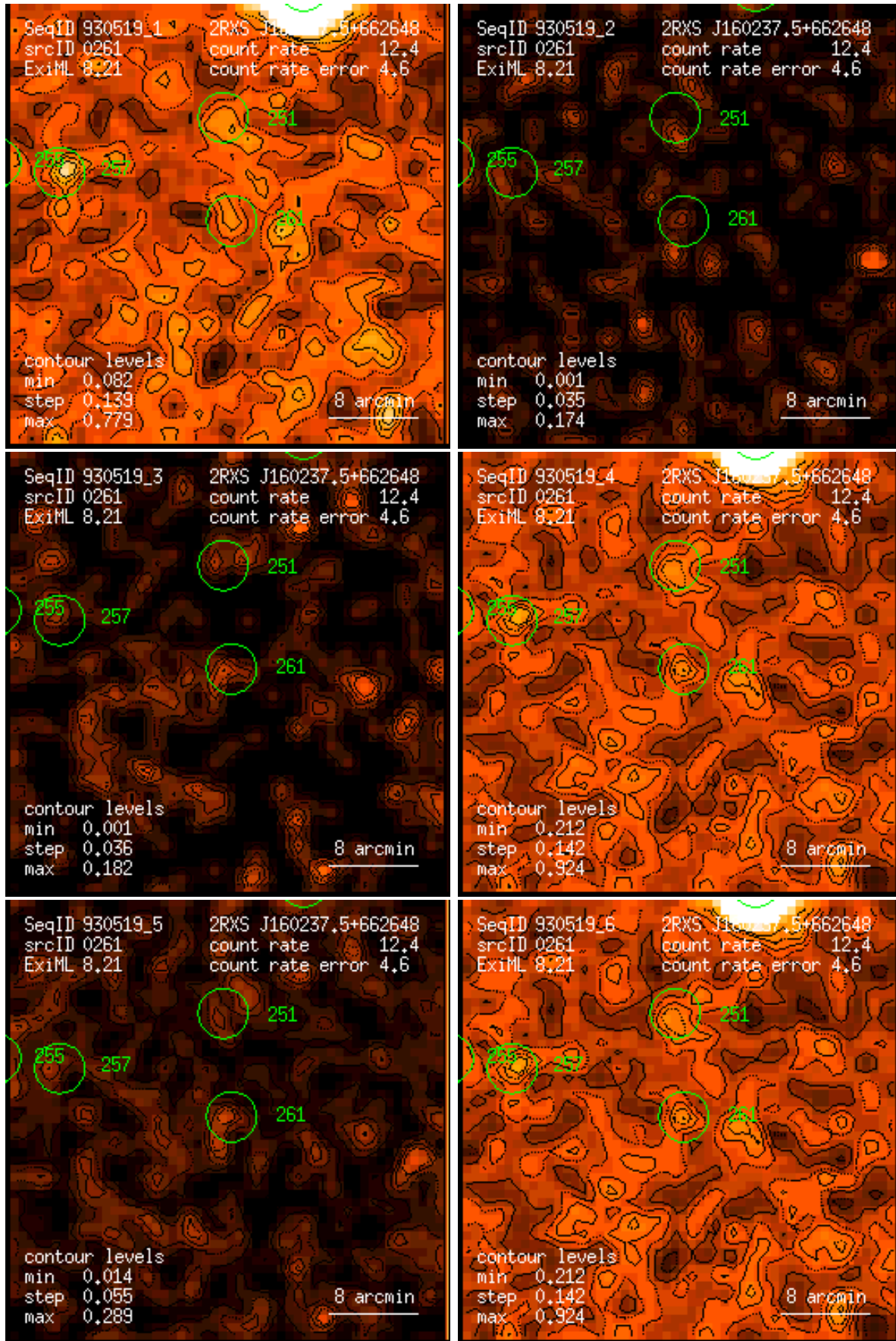
Figure 261: RASS 930519: detection 0261: band rate images, Gaussian filter: (1) PSPC channels 11 – 41, (2) 52 – 90, (3) 91 – 201, (4) 11 – 235, (5) 52 – 201, (6) 11 – 201. Broad band rates in counts/ks. Band rate contour levels in counts/ks/arcmin 2 .
