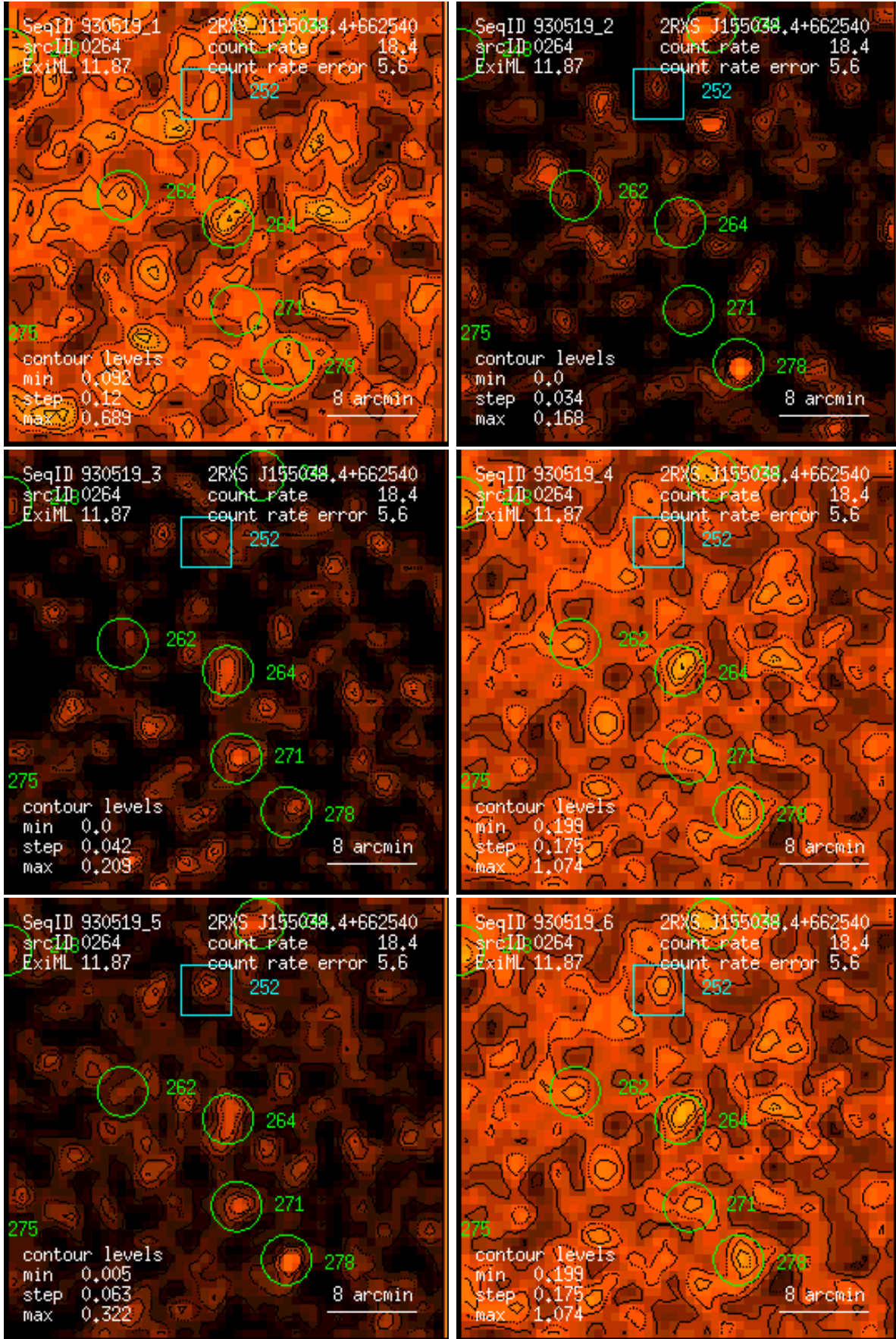
Figure 264: RASS 930519: detection 0264: band rate images, Gaussian filter: (1) PSPC channels 11 – 41, (2) 52 – 90, (3) 91 – 201, (4) 11 – 235, (5) 52 – 201, (6) 11 – 201. Broad band rates in counts/ks. Band rate contour levels in counts/ks/arcmin 2 .
