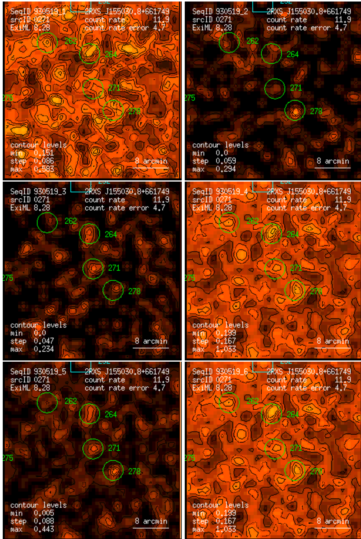
Figure 271: RASS 930519: detection 0271: band rate images, Gaussian filter: (1) PSPC channels 11 – 41, (2) 52 – 90, (3) 91 – 201, (4) 11 – 235, (5) 52 – 201, (6) 11 – 201. Broad band rates in counts/ks. Band rate contour levels in counts/ks/arcmin 2 .
